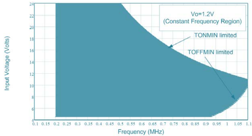
Figure 22 · Setting switching frequency correctly for V_{OUT} = 1.2V , and its safe input operating region
