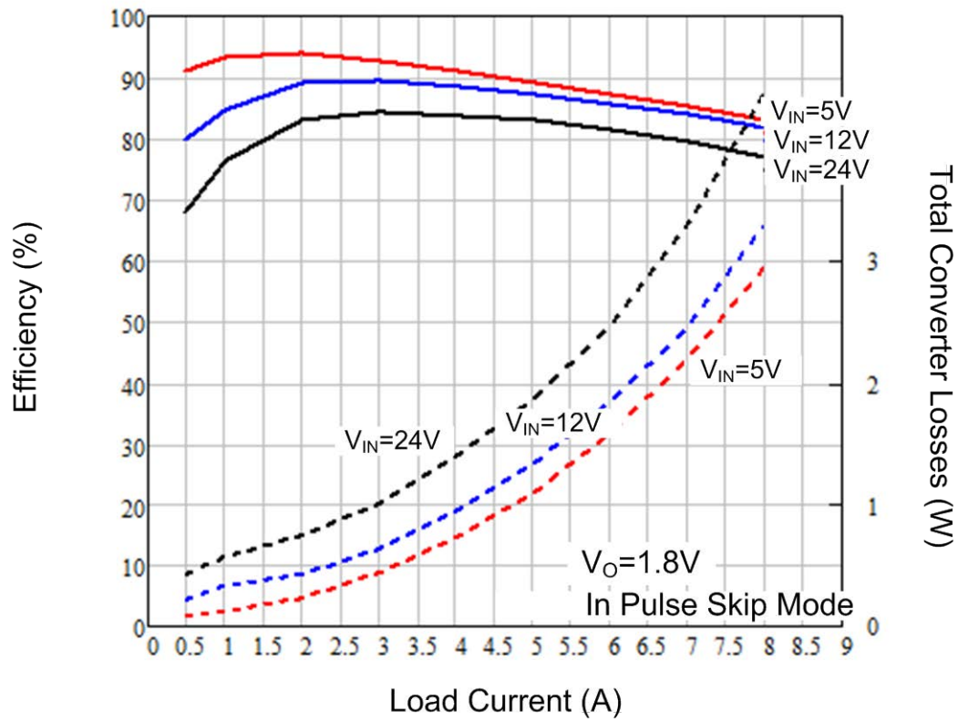
Figure 11 · Efficiency and Converter Losses in PSM Mode V_{OUT} = 1.8\text{ V} , F_s = 300\text{ kHz}
