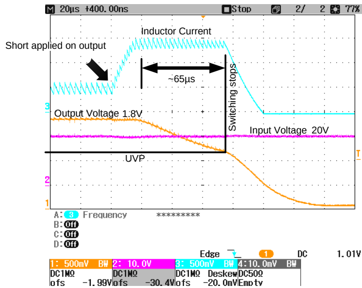
Figure 9 · Behavior under short circuit
