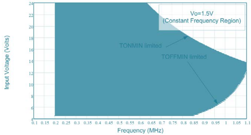
Figure 23 · Setting switching frequency correctly for V_{OUT} = 1.5V , and its safe input operating region
