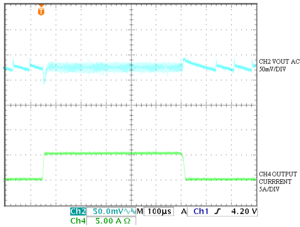
Figure 5 · Step response in PSM mode when V_{IN} = 5\text{ V}
