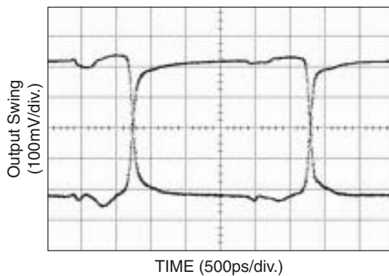
200MHz Clock
