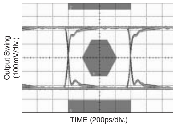
1xGBE Mask 2 23 -1
