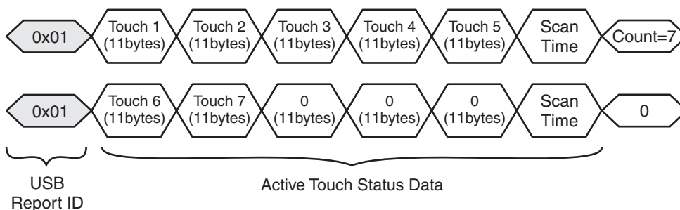
Figure 12-21. Example Input Report Packets for 7 Active Touches
