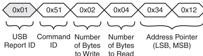
Figure 12-7. Example of a Four-byte Read Starting at Address 0x1234
