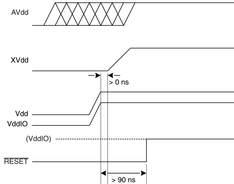
Figure 7-1. Power Sequencing on the mXT1664T2-C2U
