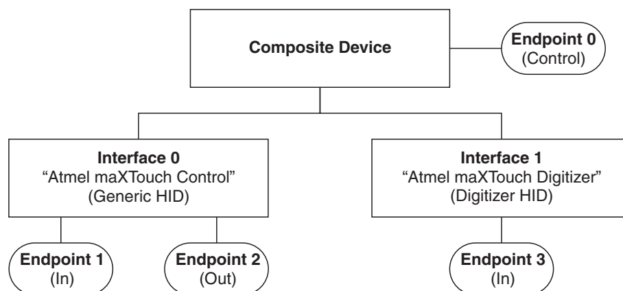
Figure 12-1.USB Topography
