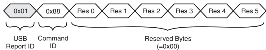
Figure 12-10.Command Packet Format
