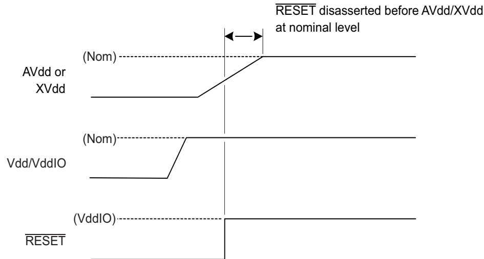
Figure 7-2. Power Sequencing on the mXT1666T2-C2U – Late rise on AVDD or XVdd
