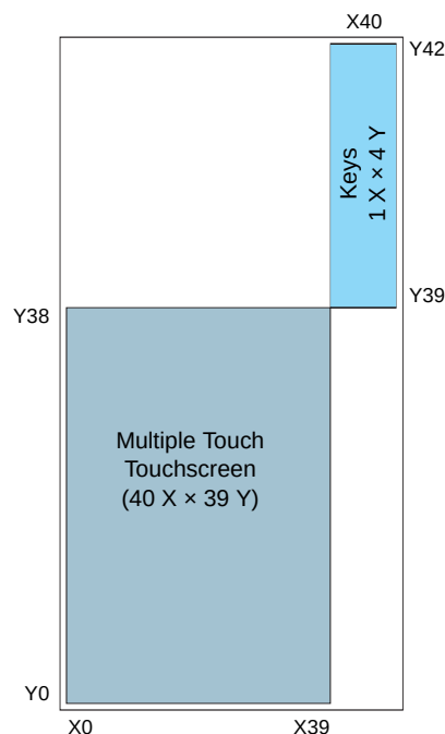
Figure 6-1. Example Layout – Optimal Cycle Time
