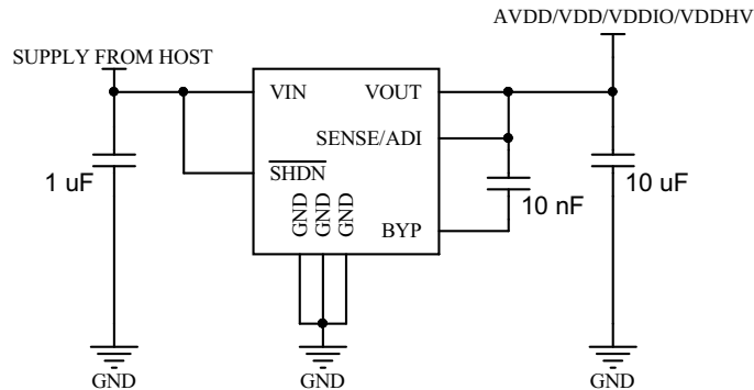
Figure 3-2. Low Drop-Out Regulators
