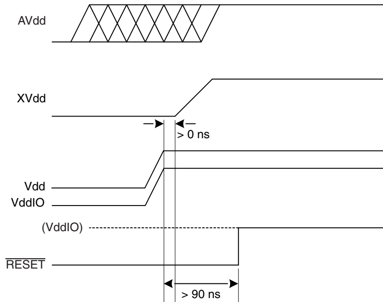
Figure 7-1. Power Sequencing on the mXT1666T2-C2U
