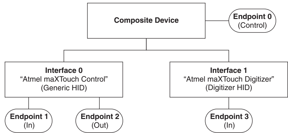
Figure 12-1.USB Topography
