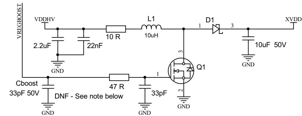
Figure 3-3. XVdd Supply Circuit
