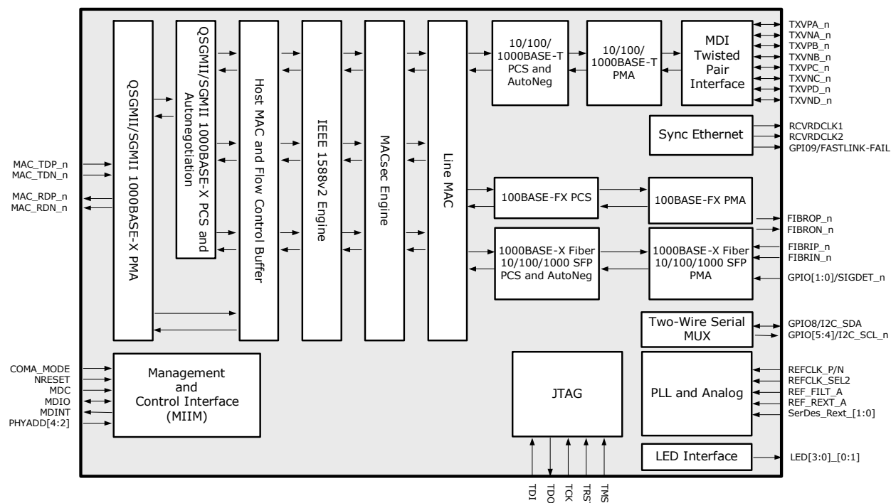
Figure 4 • Block Diagram
