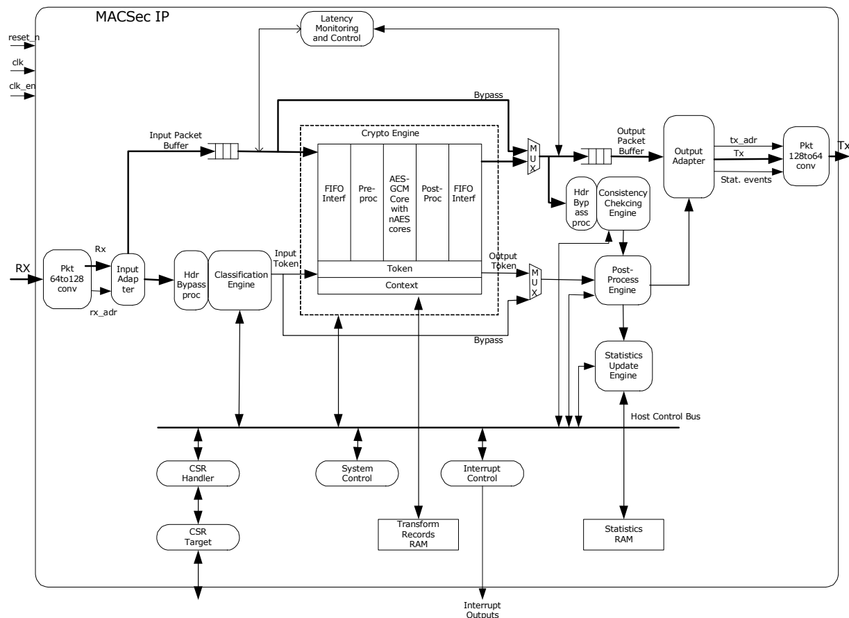
Figure 19 • MACsec Architecture
