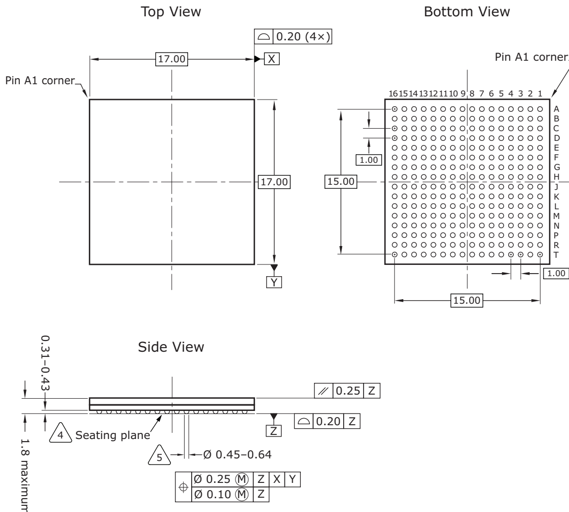
Figure 132 • Package Drawing
