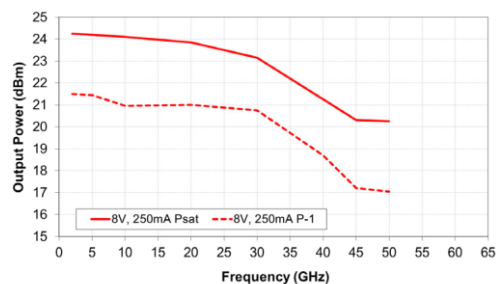
Output Power
