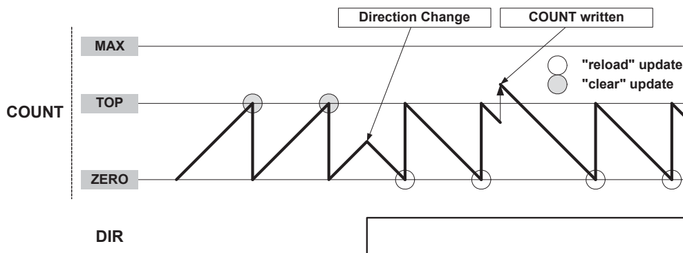
Figure 45-3. Counter Operation
