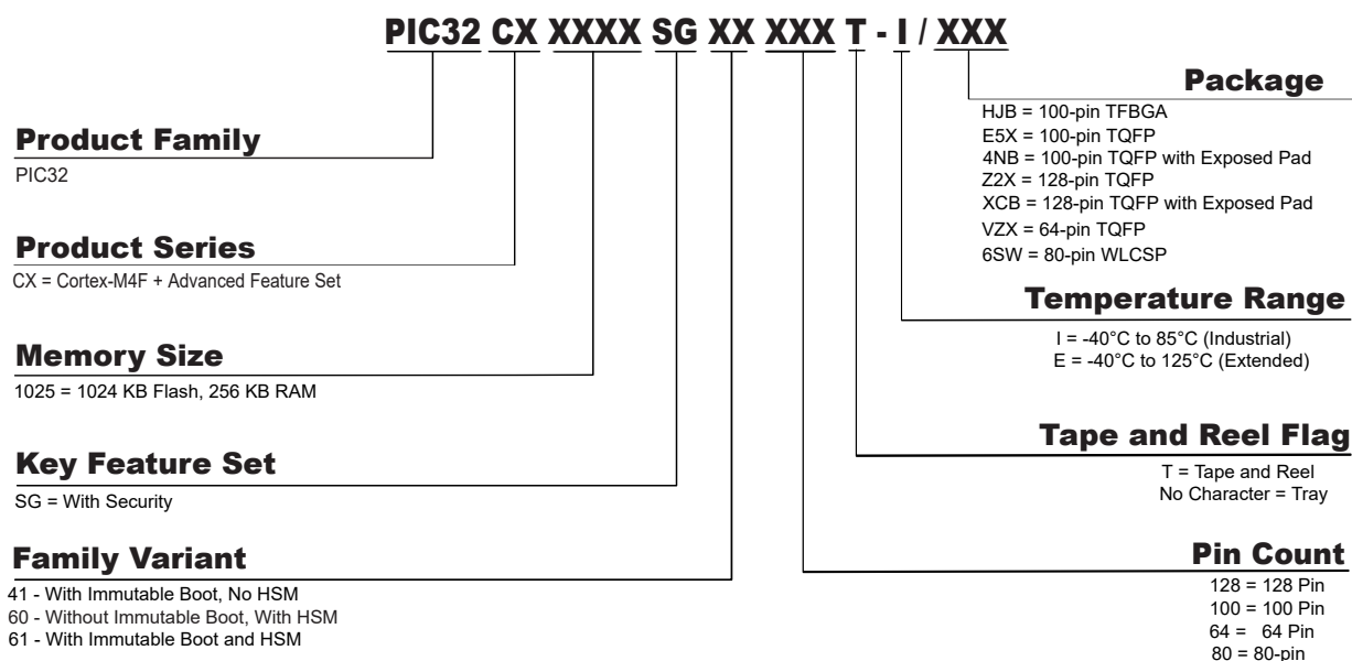
Figure 2-1. Composition of the Ordering Numbers (1,2,3)
