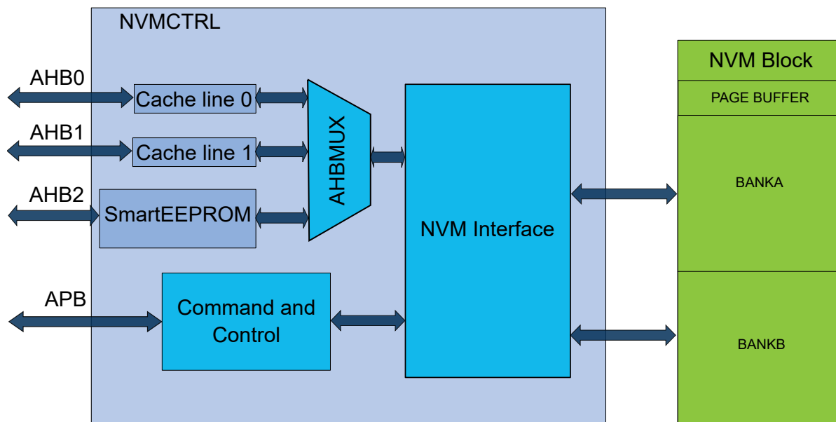
Figure 27-1. Block Diagram
