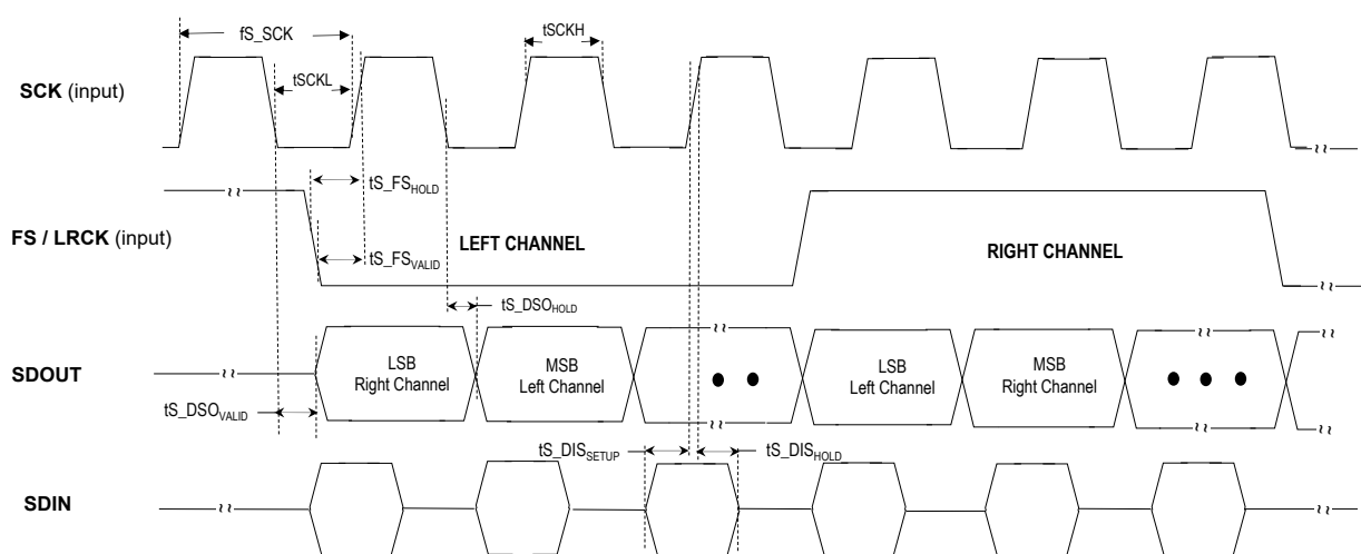
Figure 55-6. I 2 S Client Mode Timing Diagram
