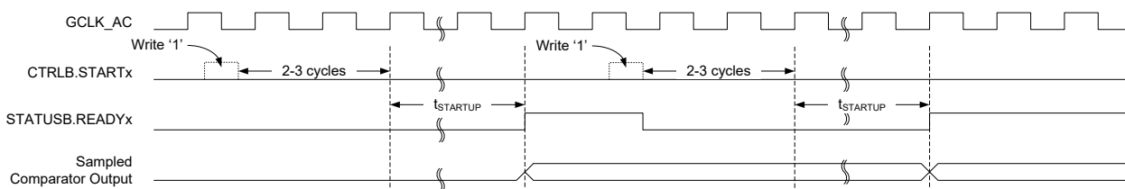
Figure 52-3. Single-Shot Example
