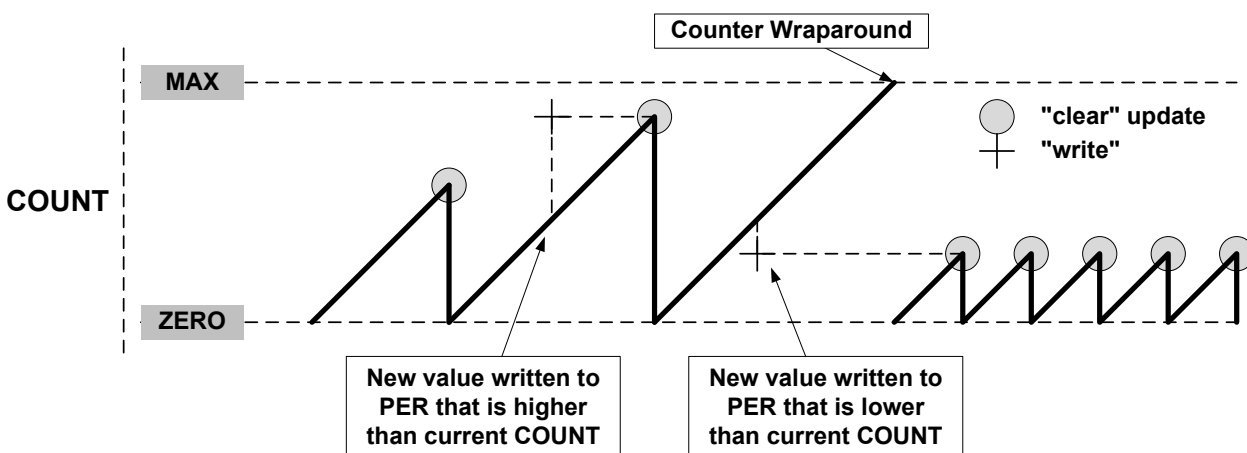
Figure 45-10. Unbuffered Single-Slope Up-Counting Operation
