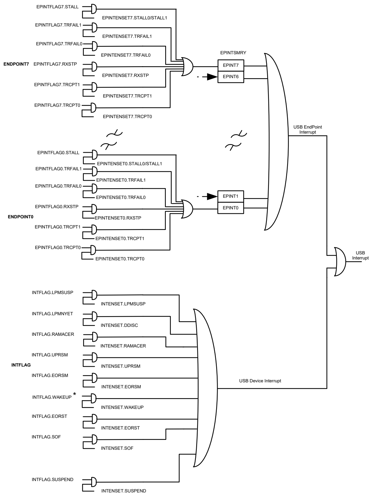
Figure 40-9. Device Interrupt
