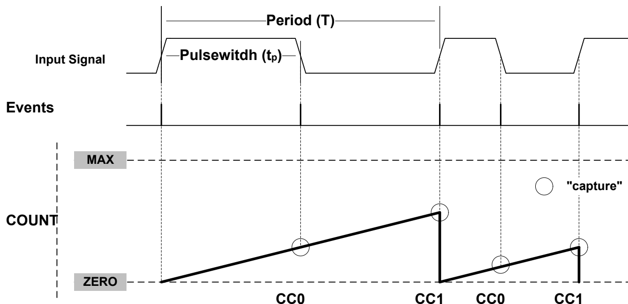
Figure 44-13. PWP Capture
