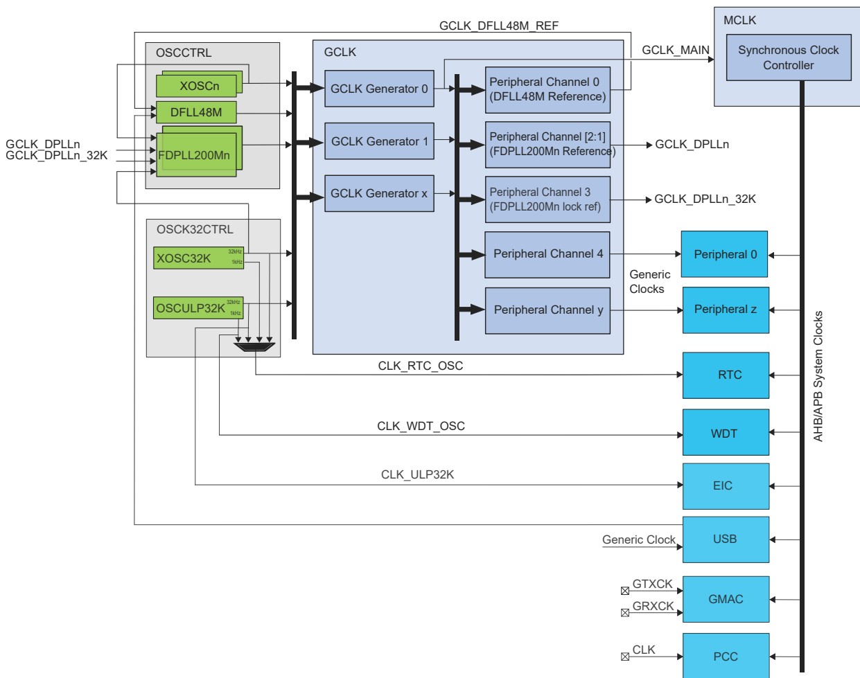
Figure 14-1. Clock Distribution
