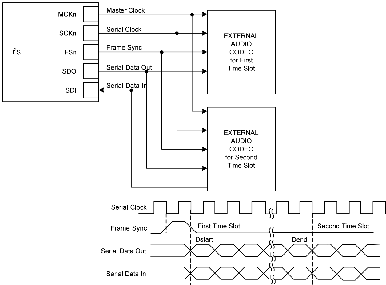
Figure 37-8. Time Slot Application Block Diagram
