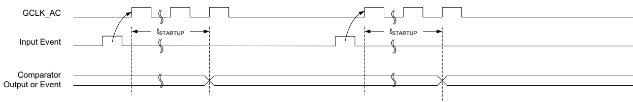
Figure 52-10. Single-Shot SleepWalking
