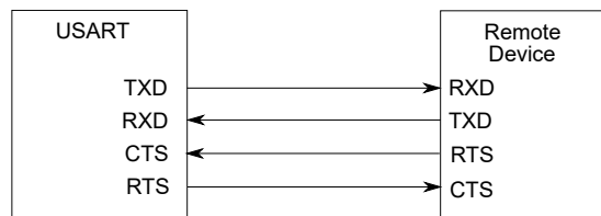
Figure 32-9. Connection with a Remote Device for Hardware Handshaking
