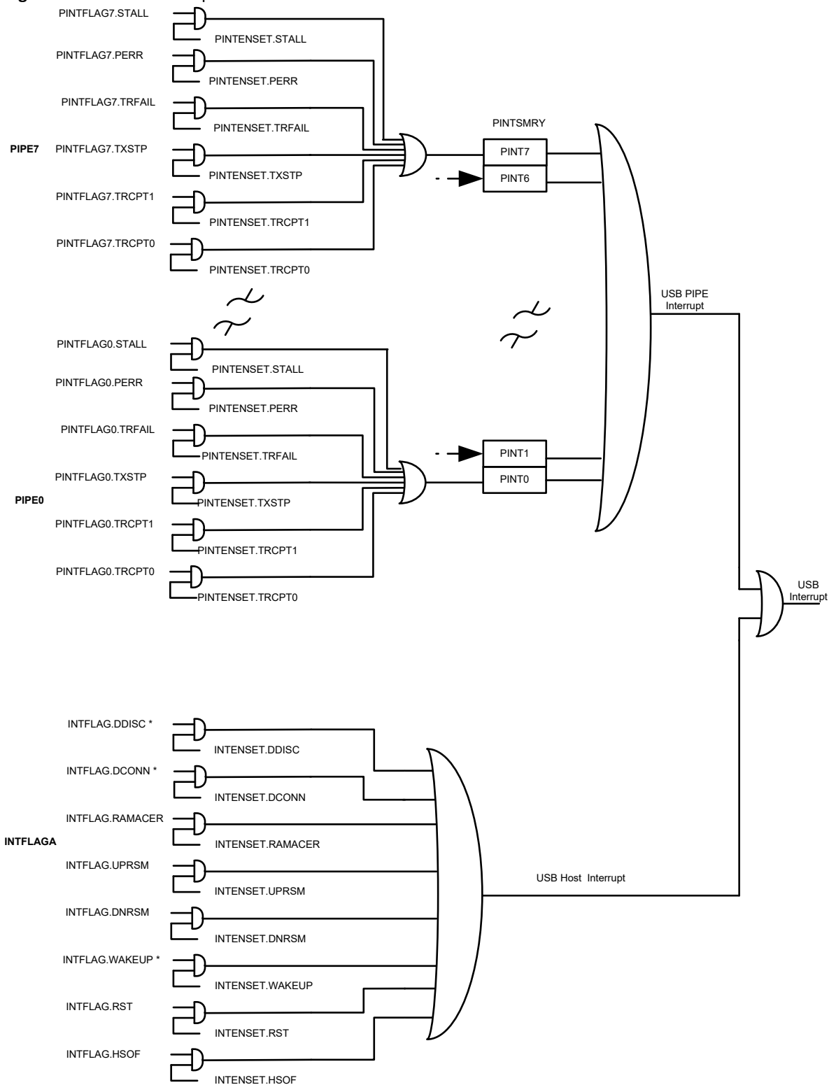
Figure 40-10. Host Interrupt
