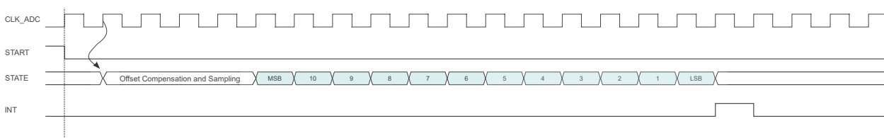
Figure 51-5. ADC Timing for One Conversion with Offset Compensation, 12-bit
