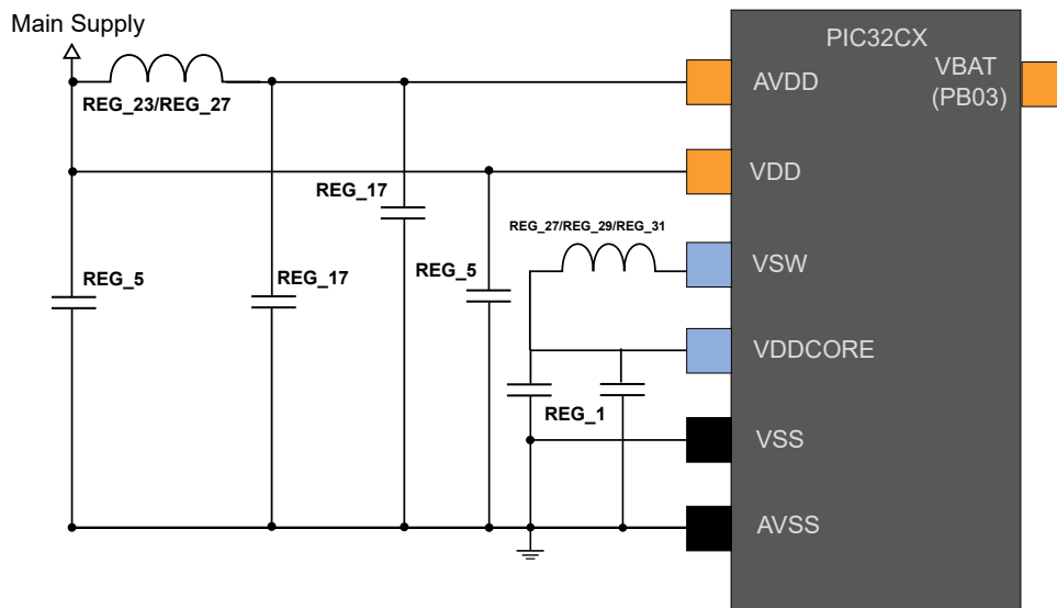
Figure 58-1. Power Supply Connection for Switching/Linear Mode
