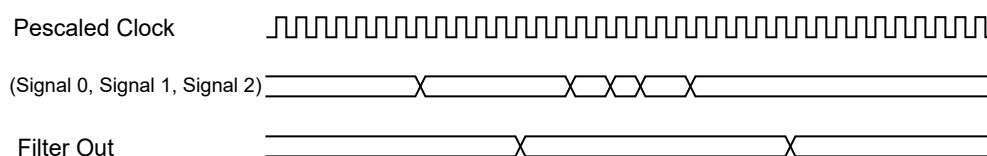
Figure 42-3. Input Signal Filtering
