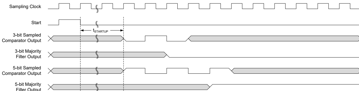
Figure 52-7. Single-Shot Filtering
