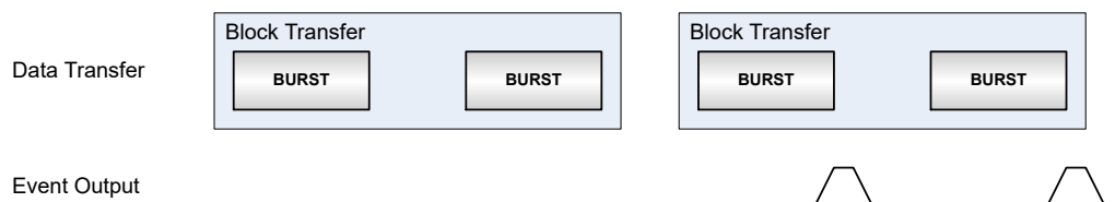
Figure 25-17. Burst Event Output Generation
