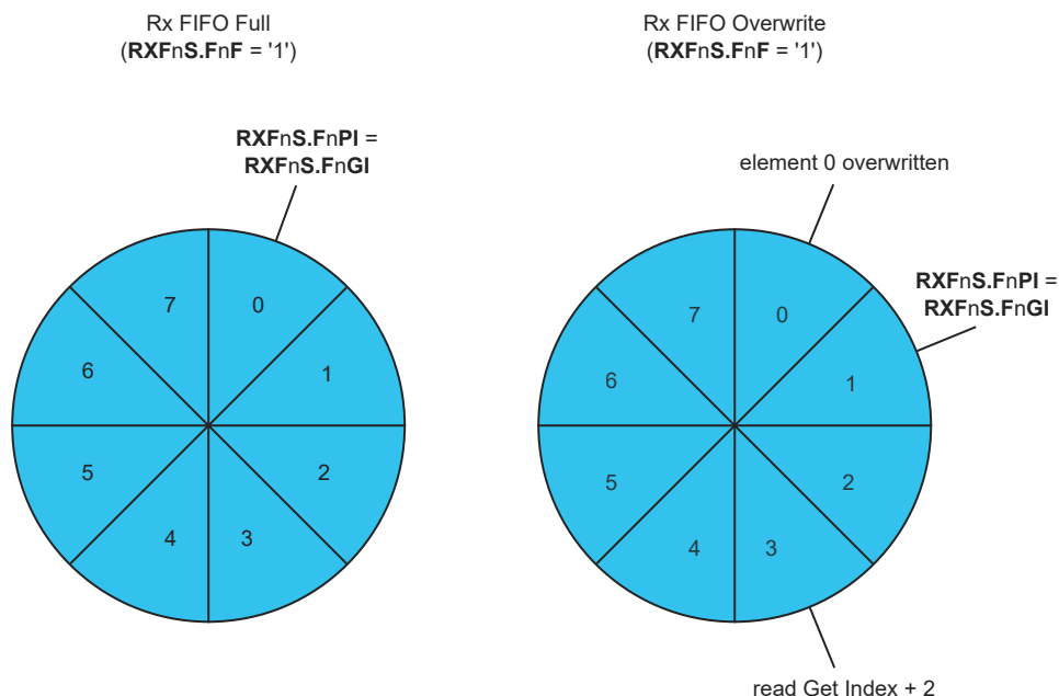
Figure 38-8. Rx FIFO Overflow Handling
