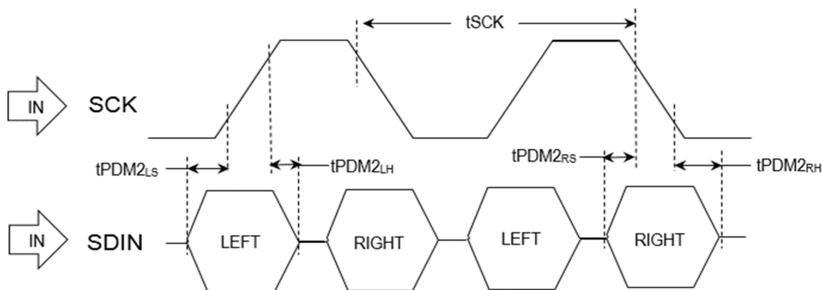
Figure 55-7. I 2 S PDM2 Mode Timing Diagram
