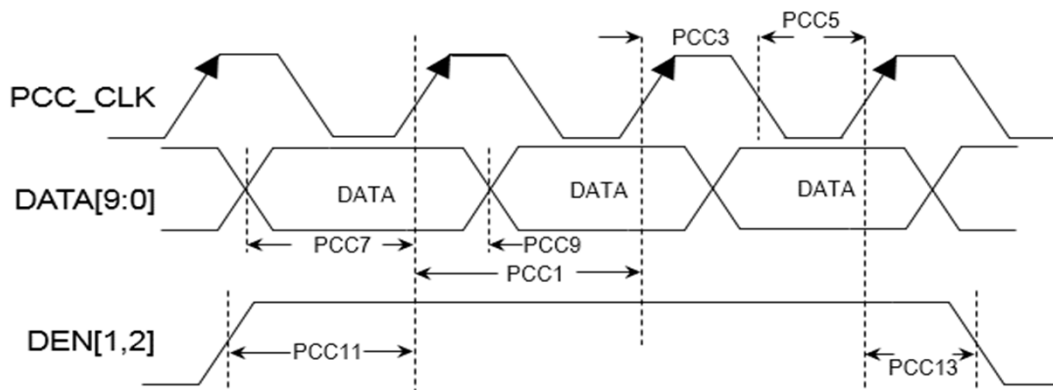
Figure 56-16. PCC Module Timing Diagram
