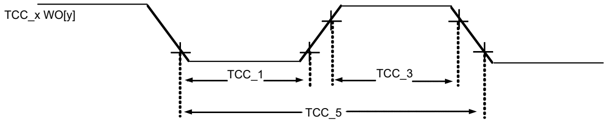
Figure 55-19. TCC Timer Compare Output Module Timing Diagrams
