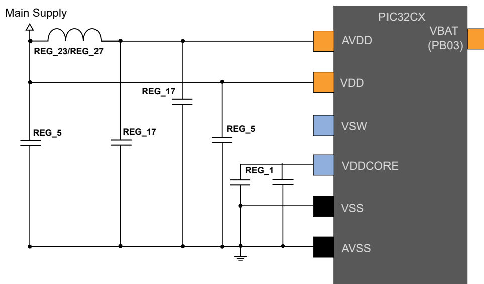
Figure 58-2. Power Supply Connection for Linear Mode Only
