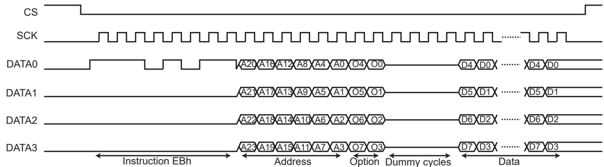
Figure 35-9. Instruction Frame
