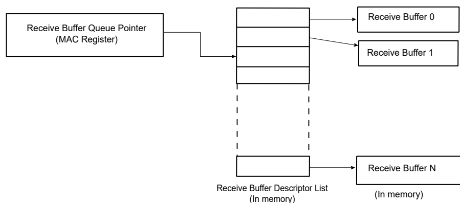
Figure 41-3. Receive Buffer List
