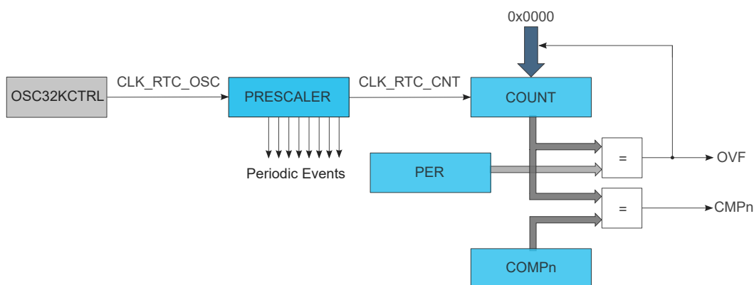
Figure 23-2. RTC Block Diagram (Mode 1 — 16-Bit Counter)
