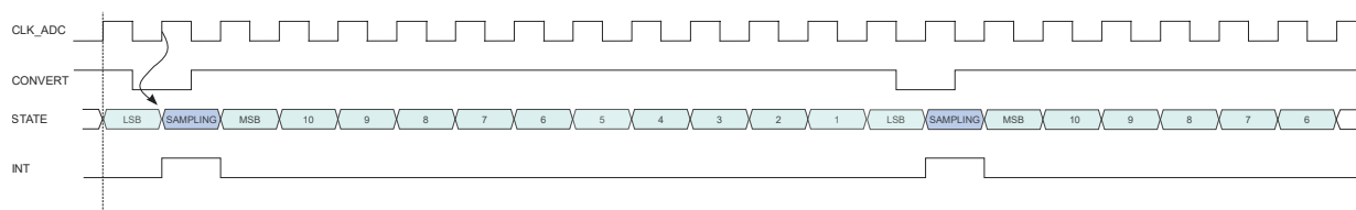
Figure 51-6. ADC Timing for Free Running in 12-bit Resolution
