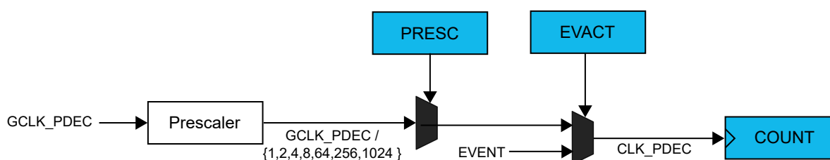
Figure 42-2. Prescaler Selection
