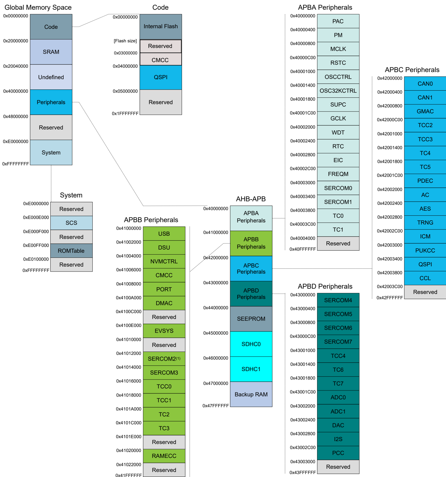
Figure 8-1. Product Mapping
