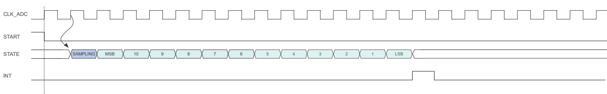
Figure 51-3. ADC Timing for One Conversion in 12-bit Resolution
