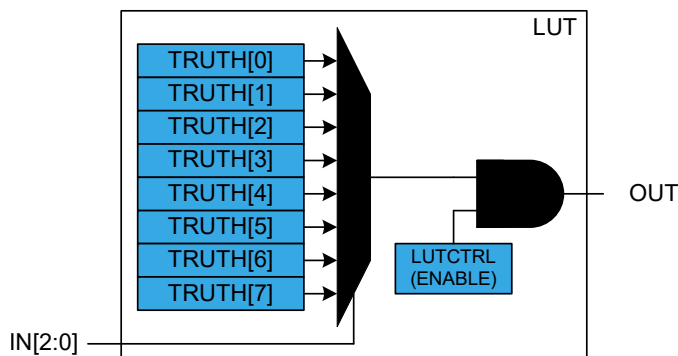
Figure 43-2. Truth Table Output Value Selection
