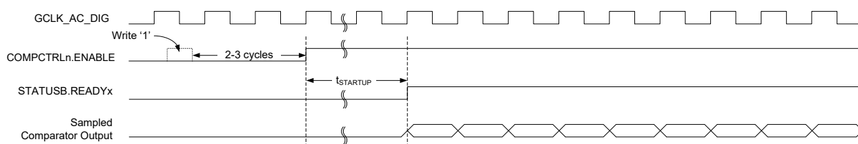
Figure 52-2. Continuous Measurement Example
