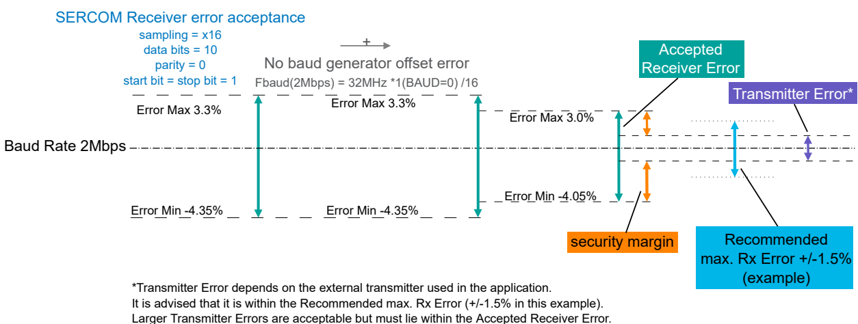
Figure 32-8. USART Rx Error Calculation Example
