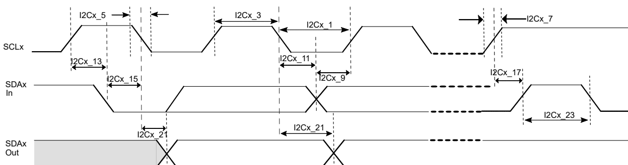
Figure 55-9. I 2 C Bus Data Host Mode Timing Diagrams
