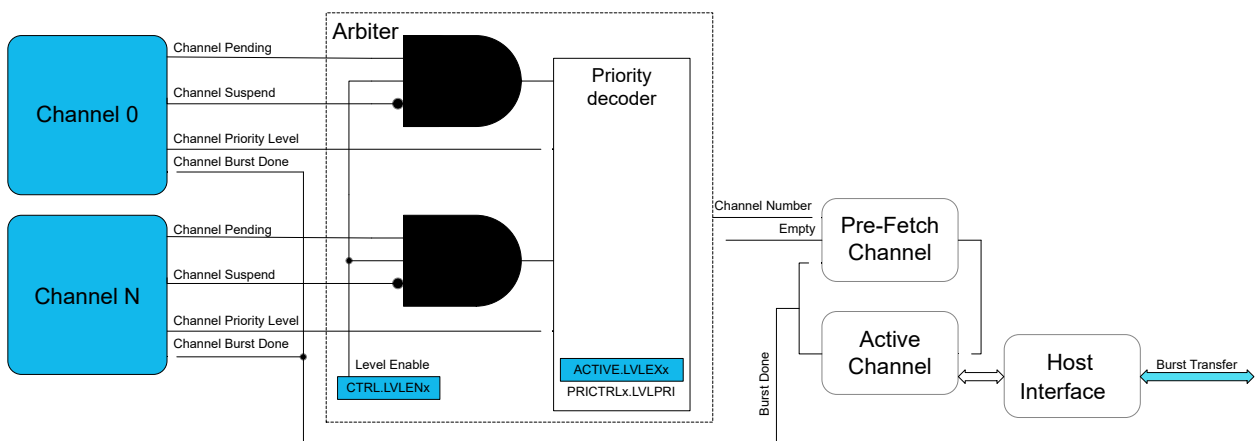
Figure 25-4. Arbiter Overview
