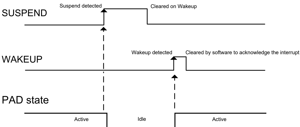
Figure 40-8. Pad Events
