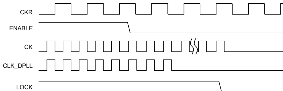
Figure 18-6. CK and CLK_DPLL Output from Running Mode to DPLL Off Mode.
