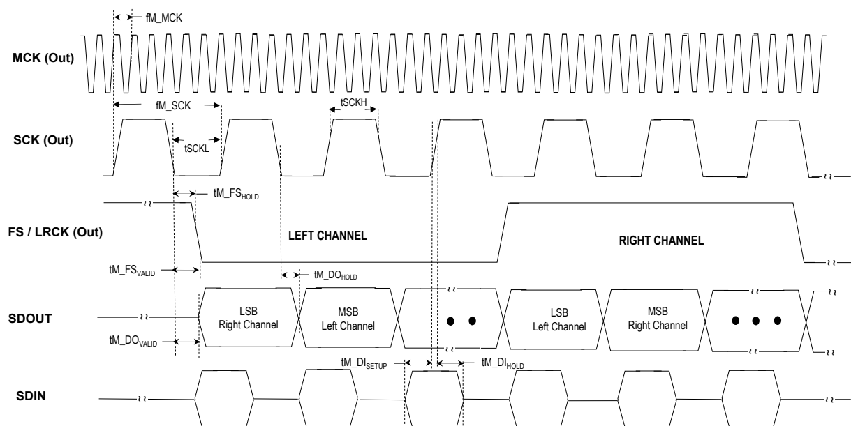
Figure 55-5. I 2 S Host Mode Timing Diagram
