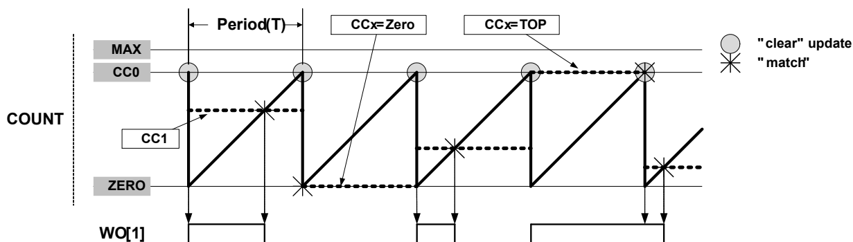
Figure 44-6. Match PWM Operation
