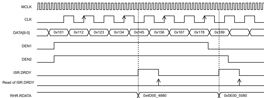
Figure 39-14. PCC Waveforms (ISIZE = 10_BITS, DSIZE = 2_DATA, ALWAYS = 0, HALFS = 1, FRSTS = 1, SCALE = 1)
