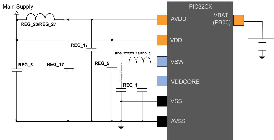
Figure 58-3. Power Supply Connection for Battery Backup Mode
