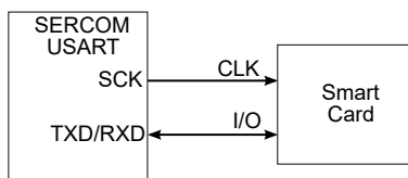
Figure 32-19. Connection of a Smart Card to the SERCOM USART
