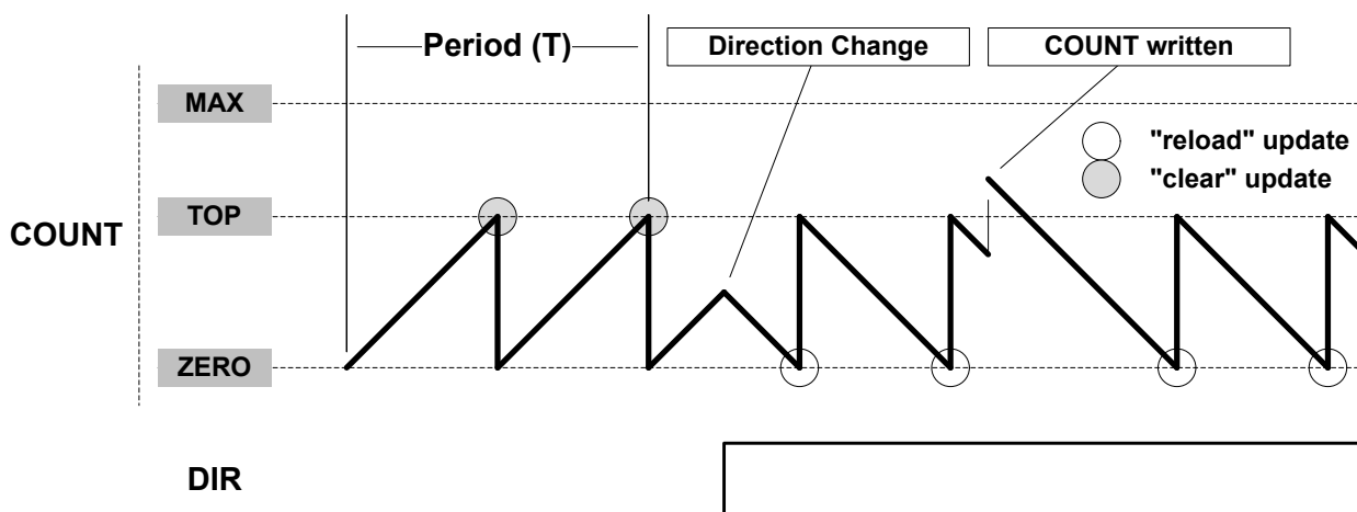
Figure 44-3. Counter Operation
