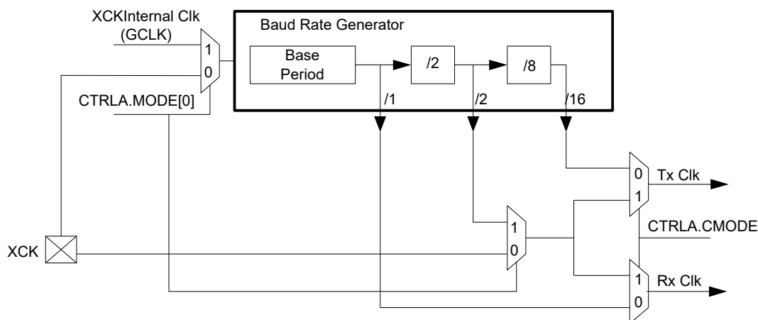
Figure 32-3. Clock Generation
