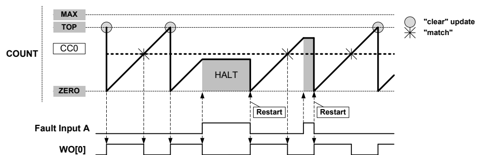
Figure 45-31. Waveform Generation with Fault Qualification, Halt, and Restart Actions
