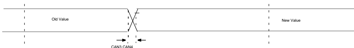
Figure 55-15. CAN Module Timing Diagram
