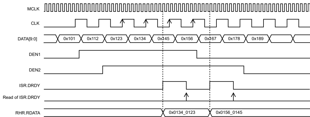
Figure 39-4. PCC Waveforms (ISIZE = 10_BITS, DSIZE = 2_DATA, ALWAYS = 0, HALFS = 0, SCALE = 0)
