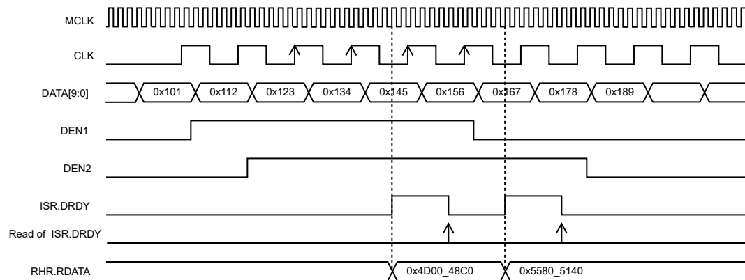
Figure 39-5. PCC Waveforms (ISIZE = 10_BITS, DSIZE = 2_DATA, ALWAYS = 0, HALFS = 0, SCALE = 1)
