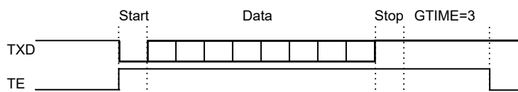
Figure 32-18. Example of TE Drive with Guard Time
