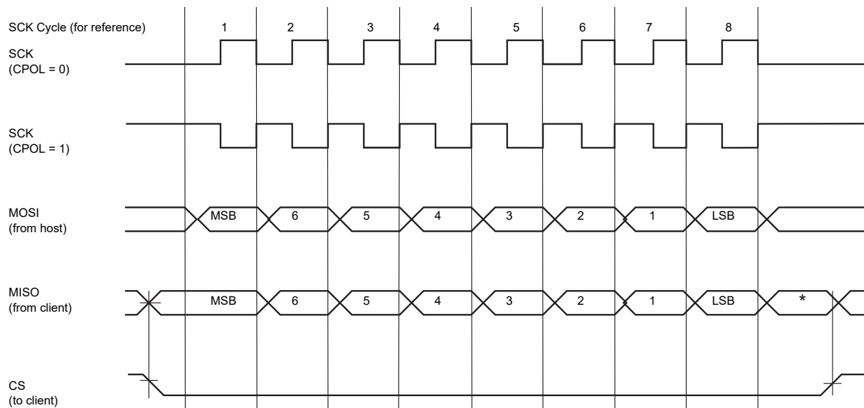
Figure 35-3. QSPI Transfer Modes (BAUD.CPHA = 0, 8-bit transfer)
