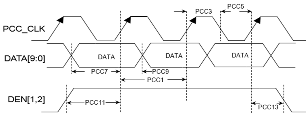
Figure 55-21. PCC Module Timing Diagram
