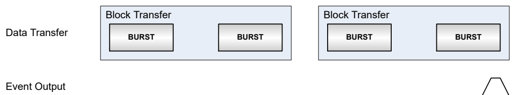
Figure 25-16. Block Event Output Generation
