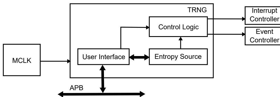
Figure 48-1. TRNG Block Diagram.
