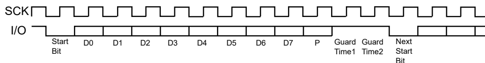
Figure 32-20. T=0 Protocol without Parity Error
