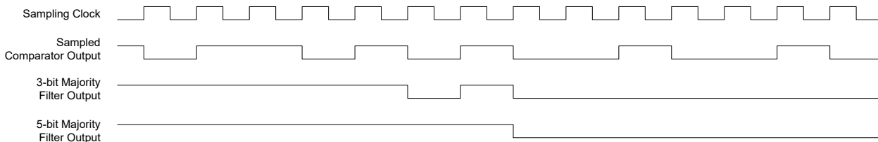
Figure 52-6. Continuous Mode Filtering
