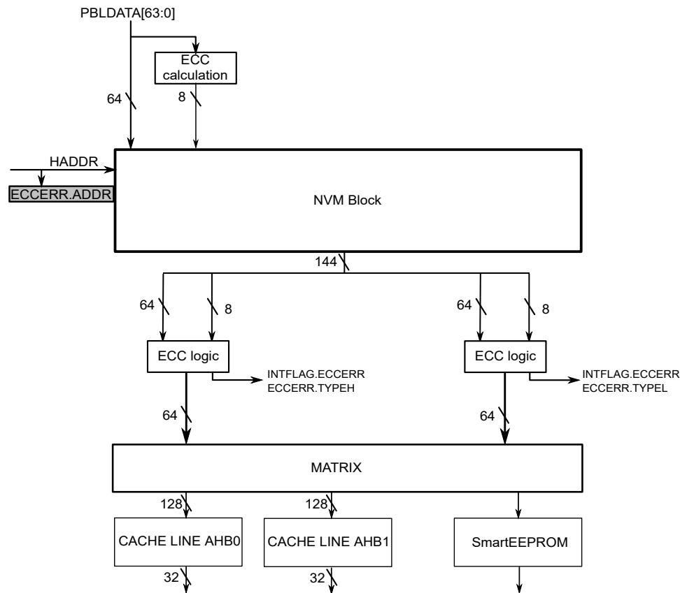
Figure 27-2. ECC Diagram
