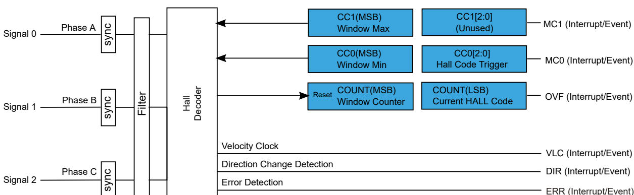
Figure 42-10. HALL Block Diagram
