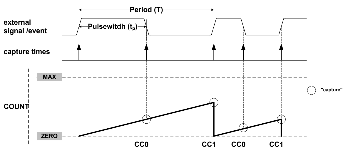
Figure 45-16. PWP Capture
