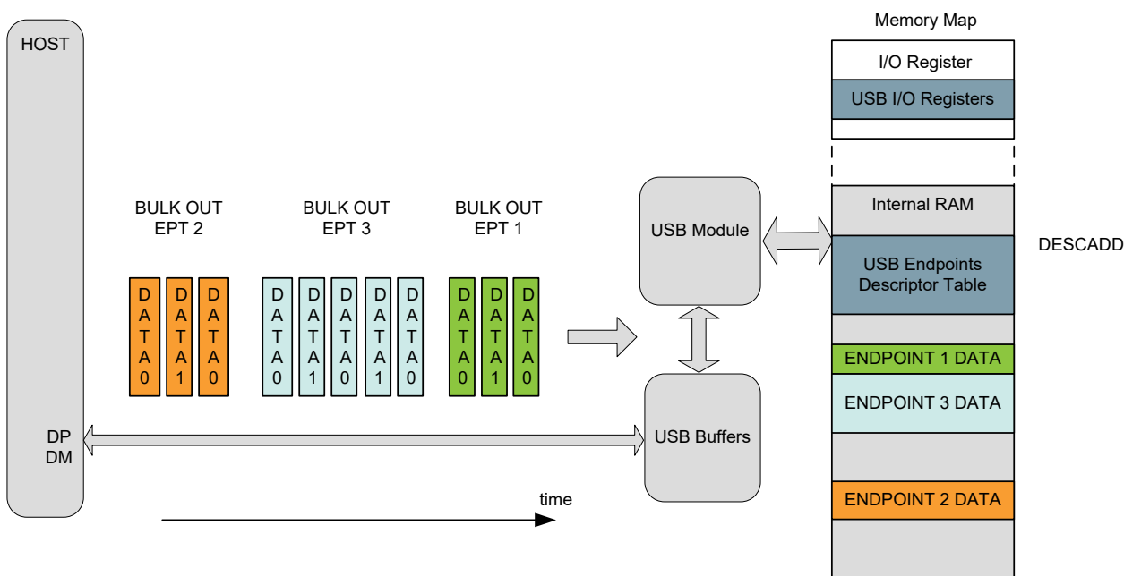
Figure 40-4. OUT Transfer: Data Packet Host to USB Device
