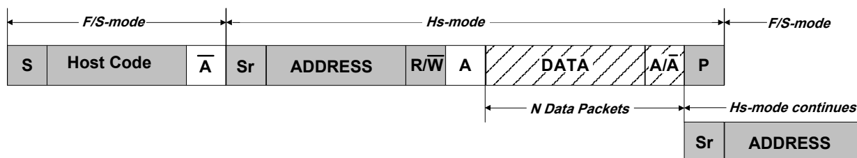
Figure 34-8. High Speed Transfer
