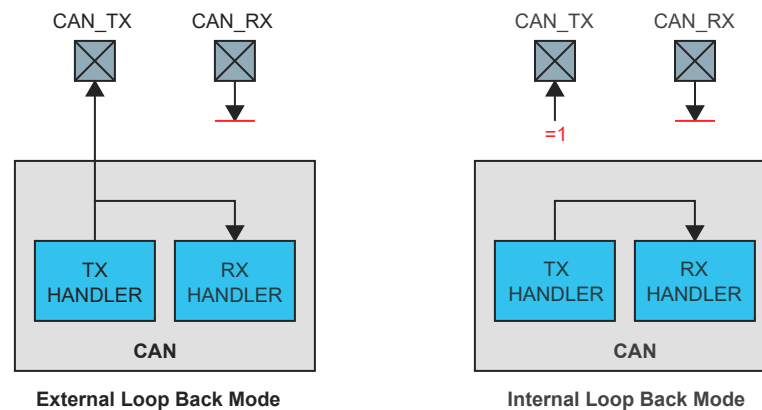
Figure 38-4. Pin Control in Loop Back Modes
