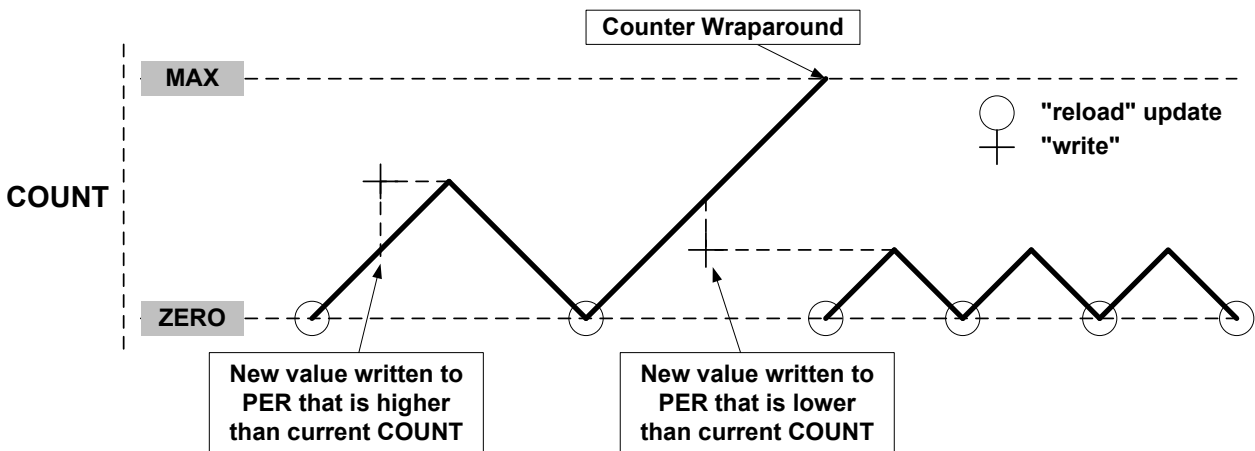
Figure 45-12. Unbuffered Dual-Slope Operation
