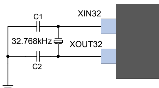
Figure 58-11. 32.768 kHz Crystal Oscillator Schematics
