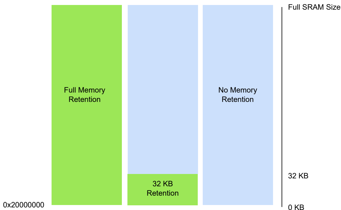
Figure 9-1. Retention Options
