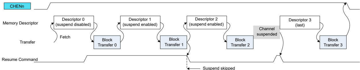
Figure 25-11. Channel Suspend/Resume Operation
