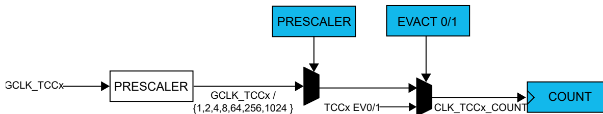
Figure 45-2. Prescaler
