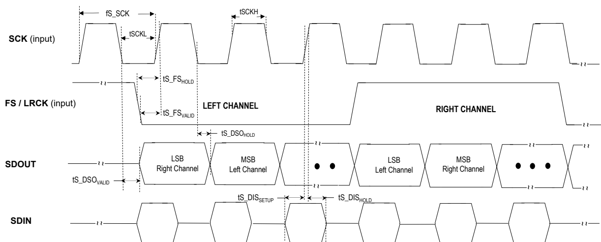
Figure 56-6. I 2 S Client Mode Timing Diagram
