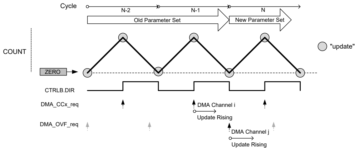
Figure 45-39. DMA Triggers in DSBOTH Operation Mode and Circular Buffer Enabled
