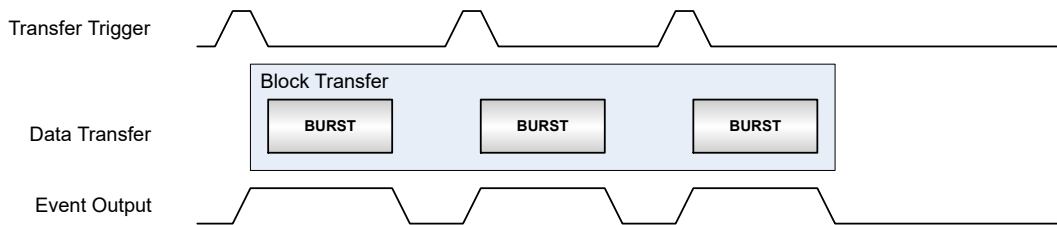
Figure 25-18. Trigger Action Event Output Generation
