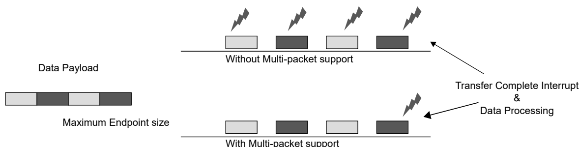
Figure 40-3. Multi-Packet Feature - Reduction of CPU Overhead
