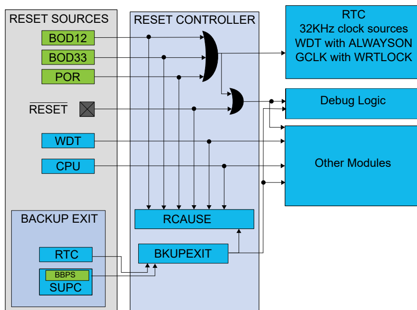
Figure 21-1. Reset System
