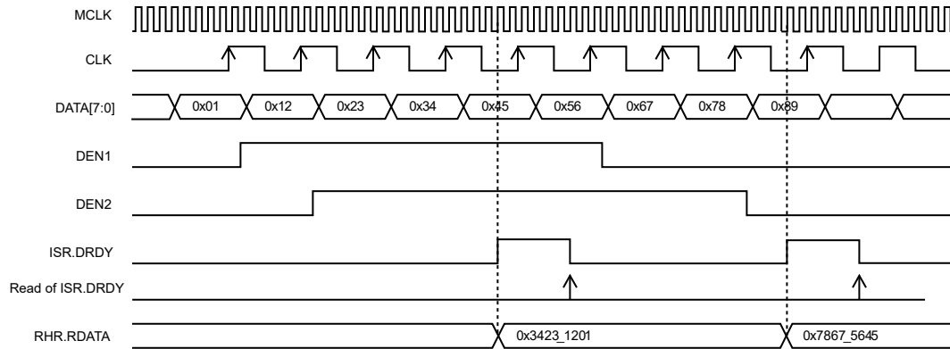
Figure 39-6. PCC Waveforms (DSIZE = 4_DATA, ALWAYS = 1, HALFS = 0)
