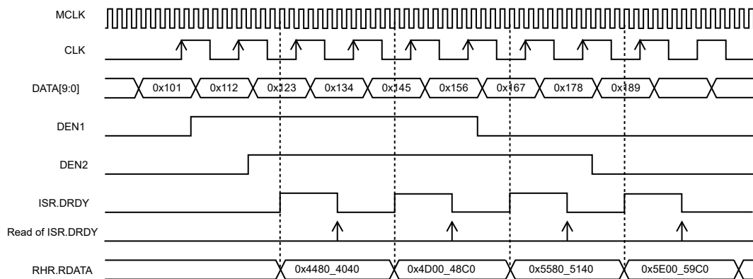
Figure 39-8. PCC Waveforms (ISIZE = 10_BITS, DSIZE = 2_DATA, ALWAYS = 1, HALFS = 0, SCALE = 1)
