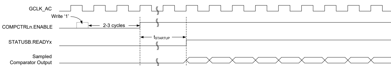
Figure 52-9. Continuous Mode SleepWalking
