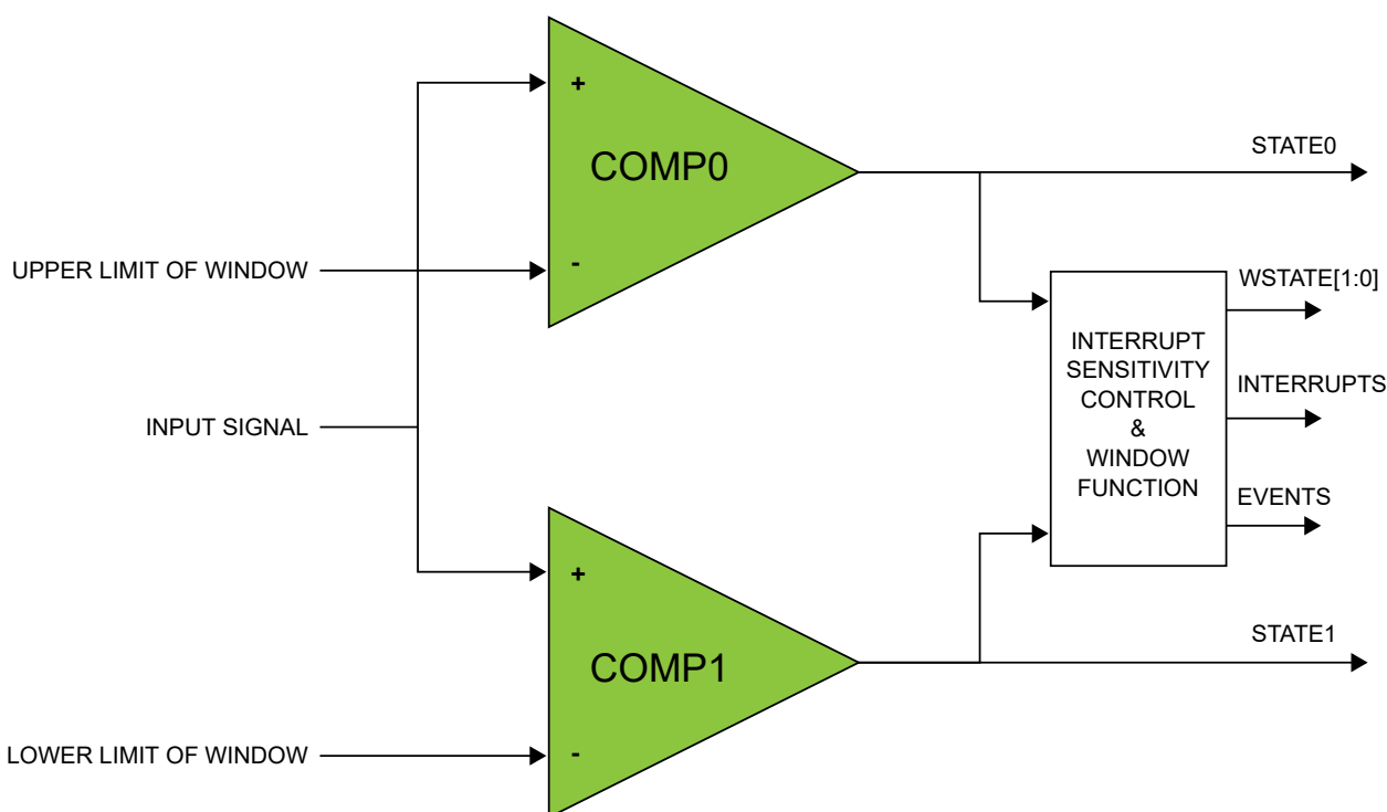
Figure 52-4. Comparators in Window Mode
