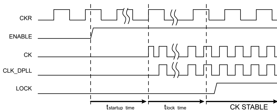
Figure 18-5. CK and CLK_DPLL Output from DPLL Off Mode to Running Mode When Wake Up Fast is Activated
