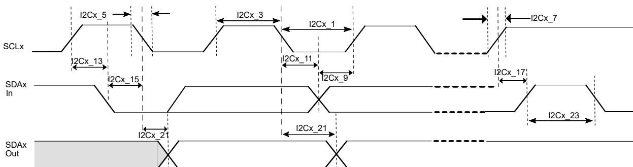
Figure 55-11. I 2 C Bus Data Client Mode Timing Diagrams
