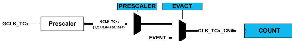
Figure 44-2. Prescaler
