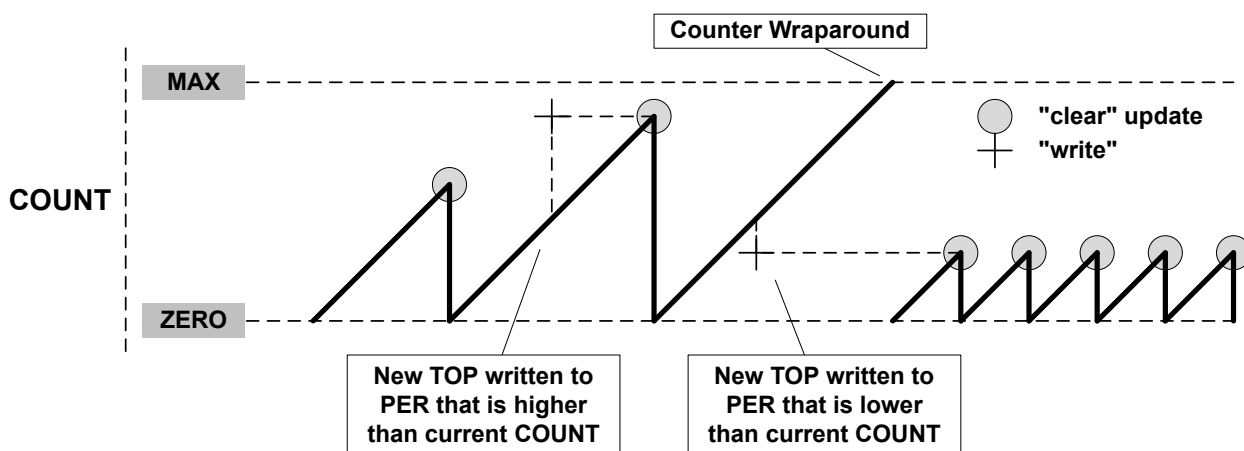
Figure 44-8. Unbuffered Single-Slope Up-Counting Operation
