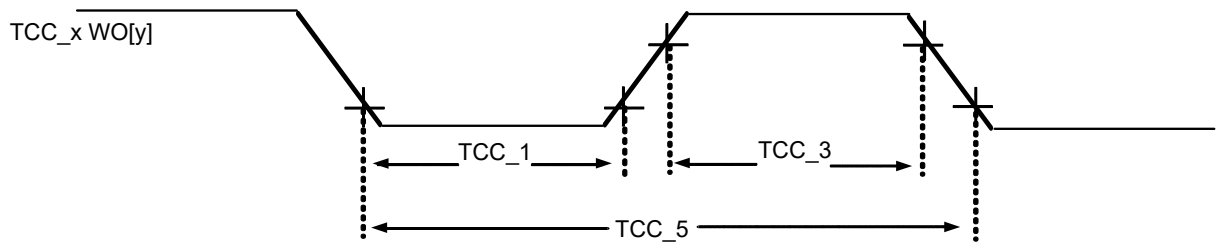
Figure 56-14. TCC Timer Compare Output Module Timing Diagrams
