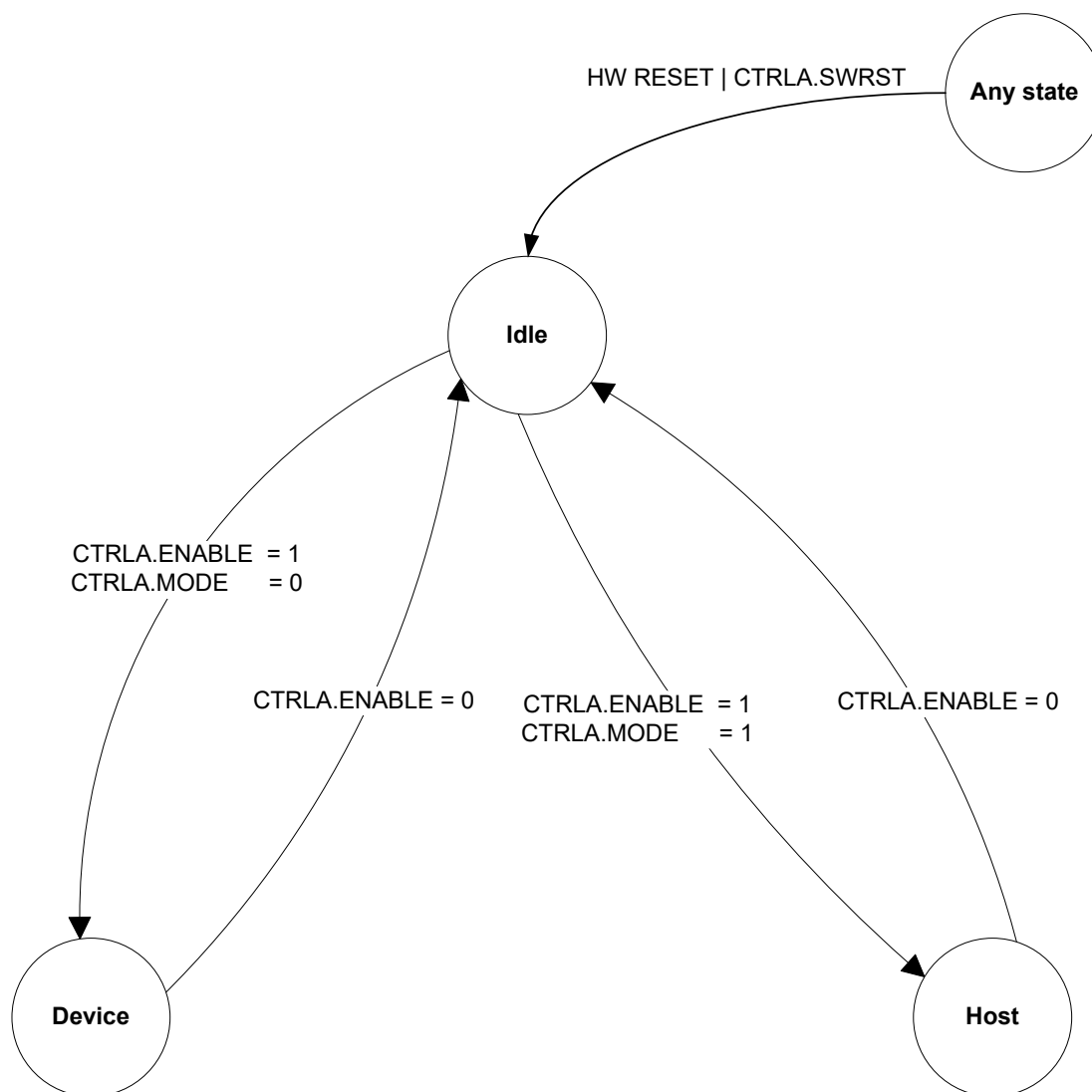
Figure 40-2. General States
