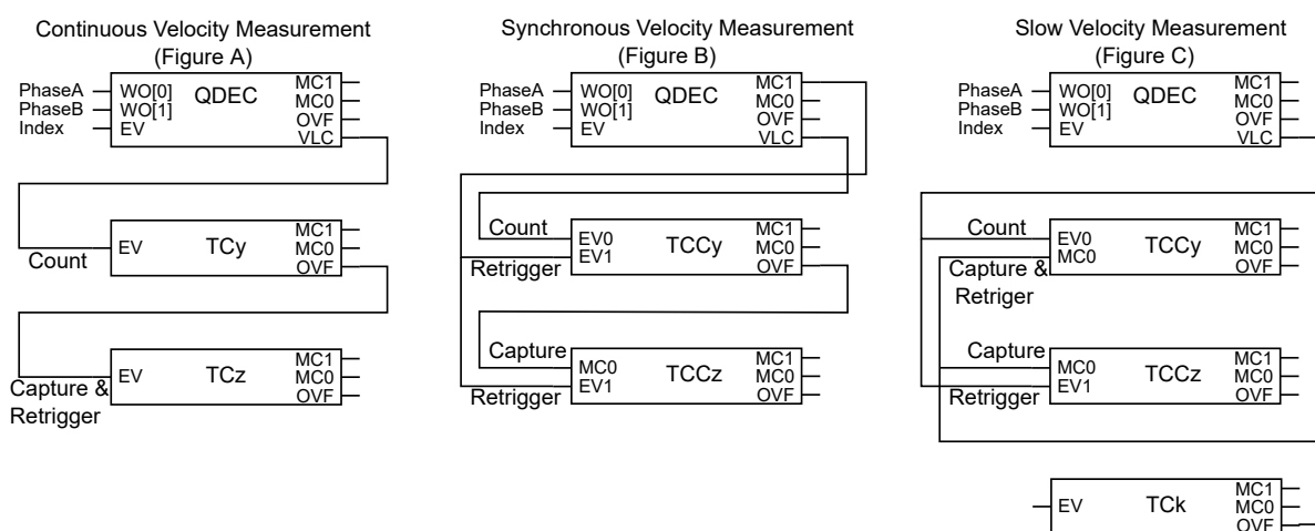
Figure 42-9. Speed Measurement
