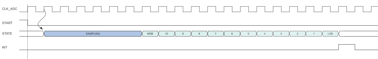
Figure 51-4. ADC Timing for One Conversion with Increased Sampling Time, 12-bit
