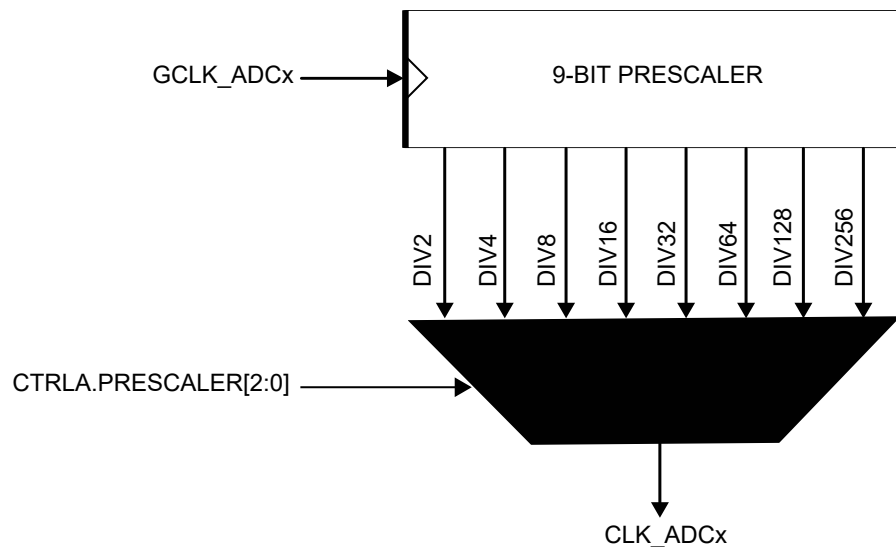
Figure 51-2. ADC Prescaler
