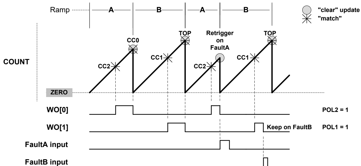
Figure 45-20. RAMP2 Critical Operation With More Than 2 Channels
