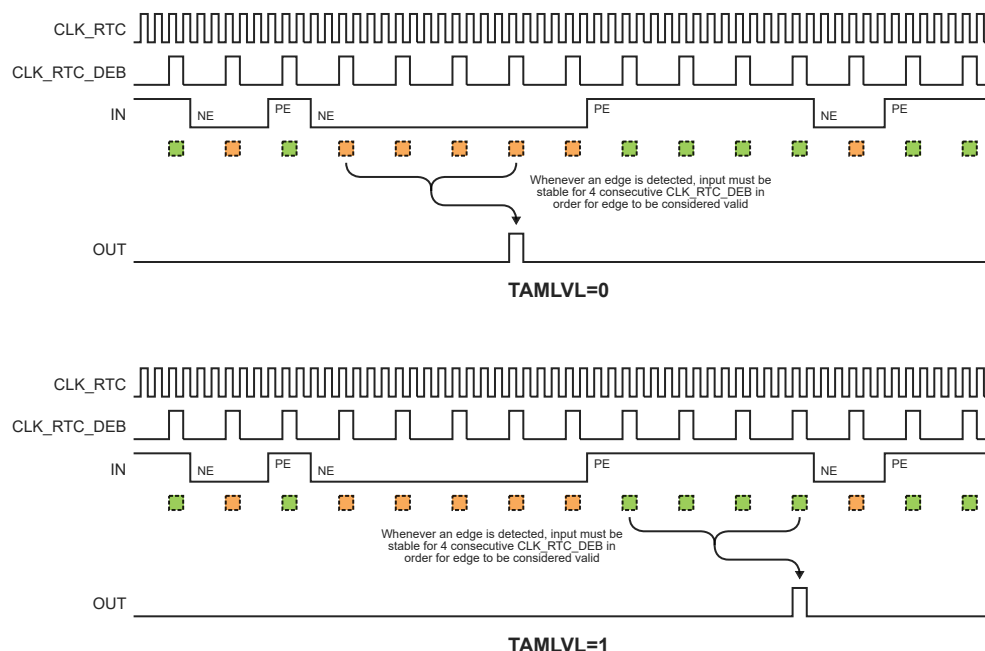
Figure 23-7. Edge Detection with Asynchronous Stability Debouncing
