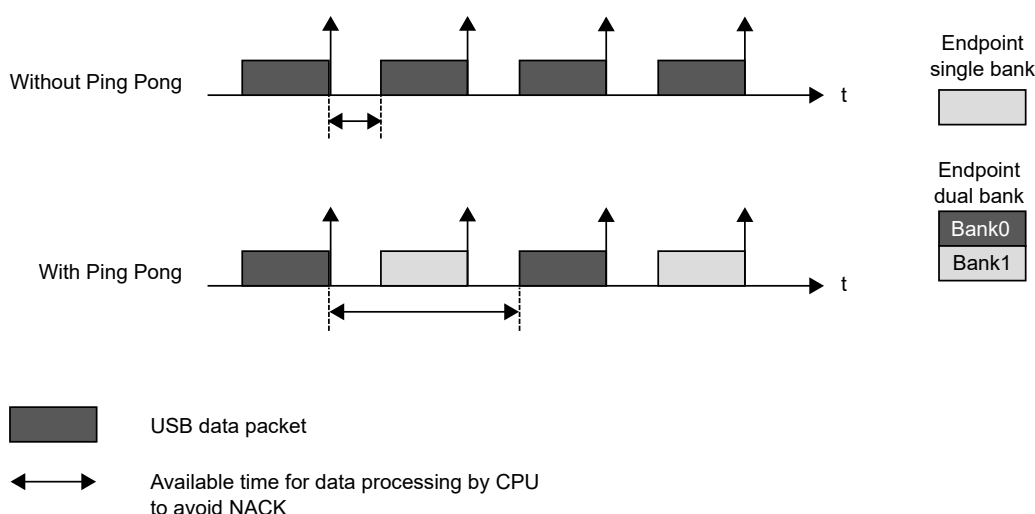
Figure 40-6. Ping-Pong Overview
