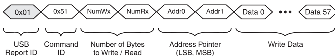
Figure 6-6. Generic Command Packet Form
