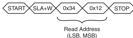
Figure 5-3. Example of a Four-byte Read Starting at Address 0x1234
