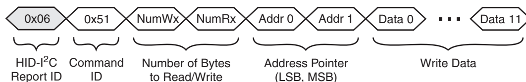
Figure 7-4. Generic Command Packet Format
