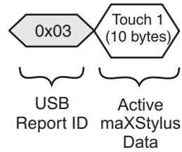
Figure 6-4. Active maXStylus Report Packet
