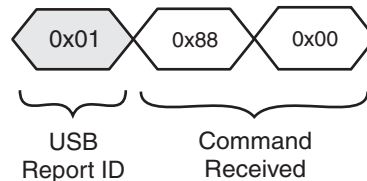
Figure 6-14. Response Packet Format
