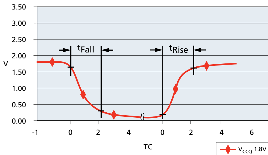
Figure 30: t_{\text{Fall}} and t_{\text{Rise}} ( V_{\text{CCQ}} = 1.7\text{-}1.95\text{V} )
