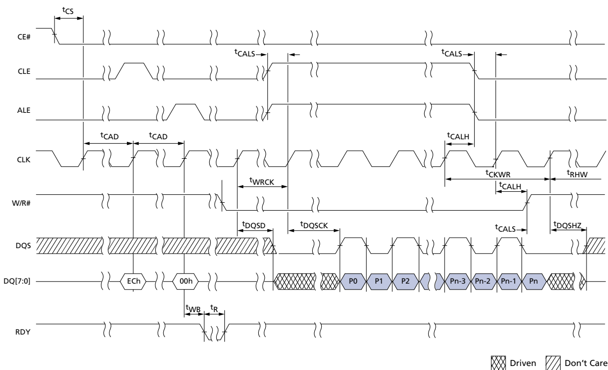
Figure 102: READ PARAMETER PAGE Operation
