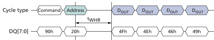
Figure 45: READ ID (90h) with 20h Address Operation
