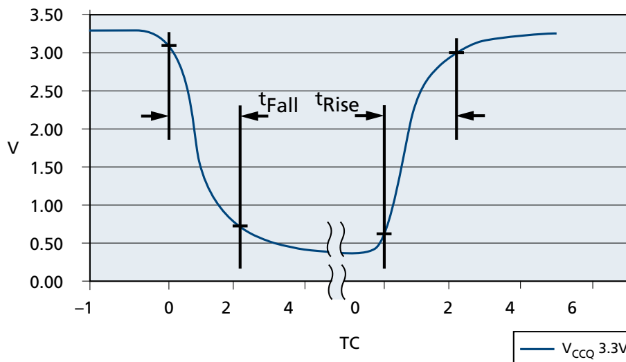
Figure 29: t_{\text{Fall}} and t_{\text{Rise}} ( V_{\text{CCQ}} = 2.7\text{-}3.6\text{V} )
