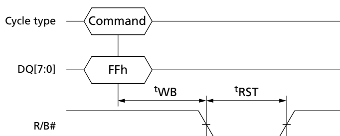
Figure 41: RESET (FFh) Operation
