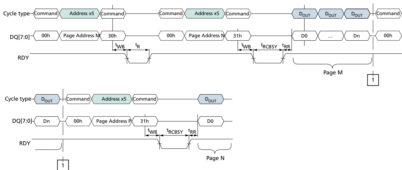
Figure 58: READ PAGE CACHE RANDOM (00h-31h) Operation
