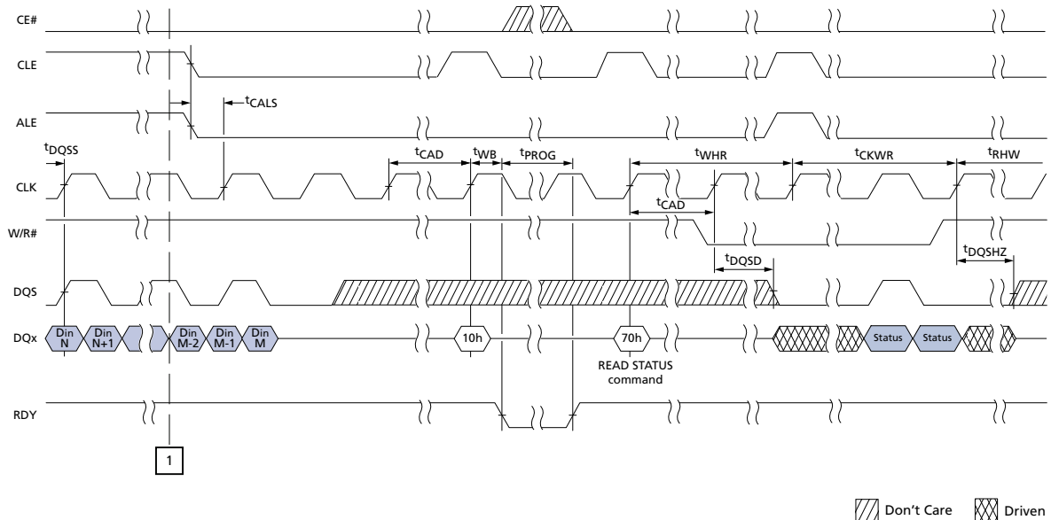
Figure 112: PROGRAM PAGE Operation (2 of 2)
