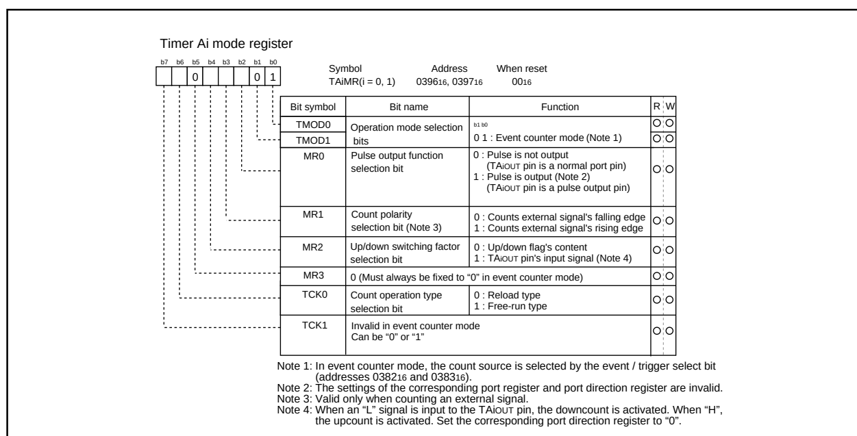
Fig.FB-8 Timer Ai mode register in event counter mode
