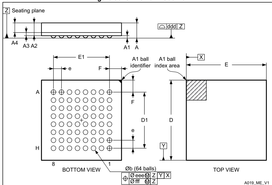
Figure 56. UFBGA64 - Outline
