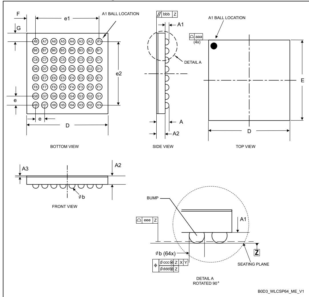
Figure 50. WLCSP64 - outline
