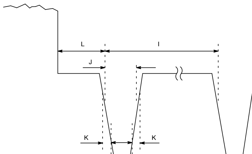
Figure 43. Equalizing Pulse
