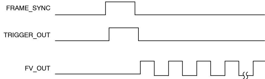
Figure 8. Continuous Mode
