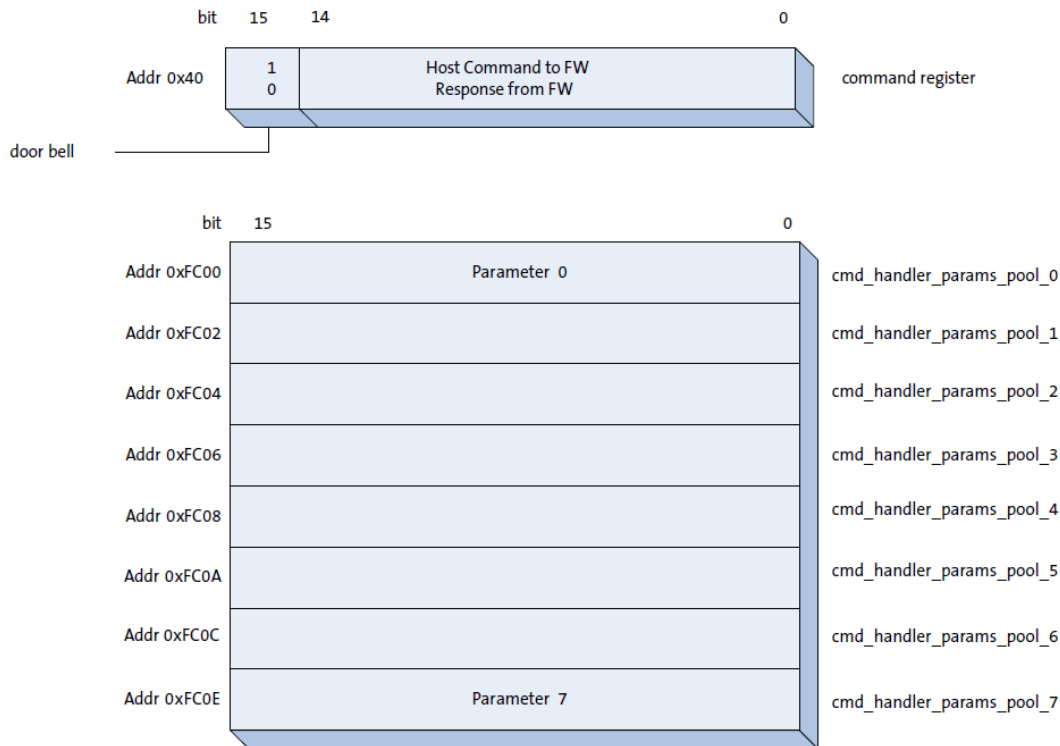
Figure 37. Interface Structure
