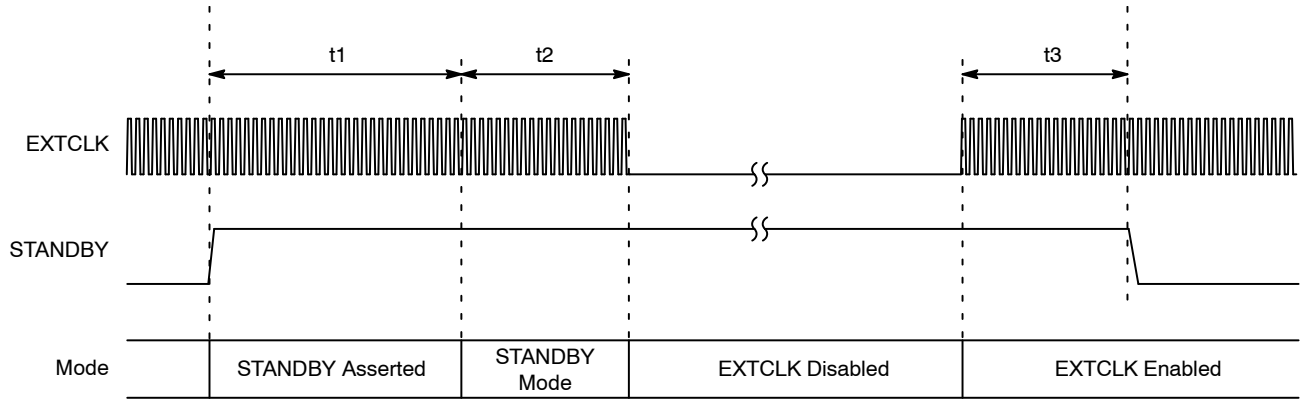
Figure 5. Hard Standby Operation
