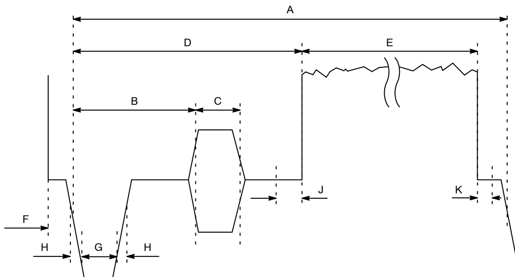
Figure 42. Video Timing
