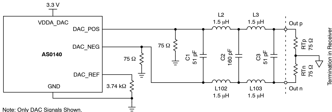
Figure 29. Differential Connection
