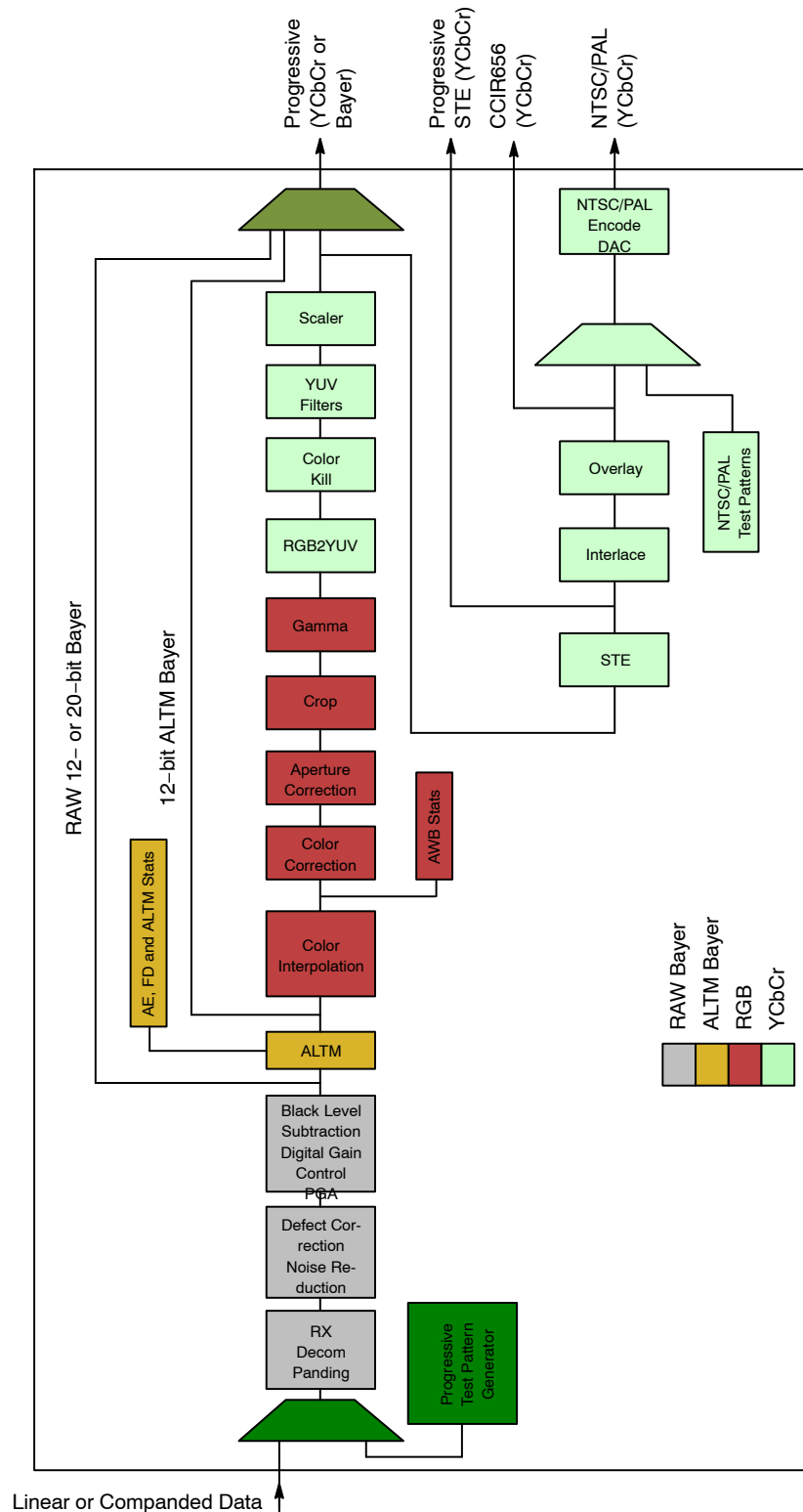
Figure 9. AS0140AT IFP
