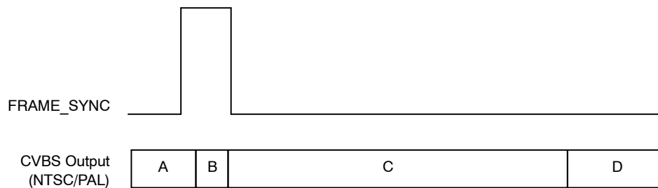
Figure 6. Frame Sync Behavior with Interlaced Mode
