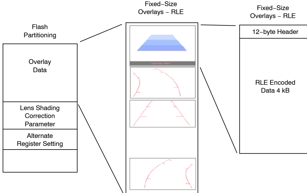
Figure 27. Memory Partitioning
