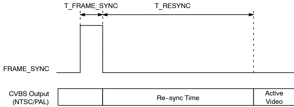
Figure 41. Frame_Sync (Interlaced Operation) Diagram
