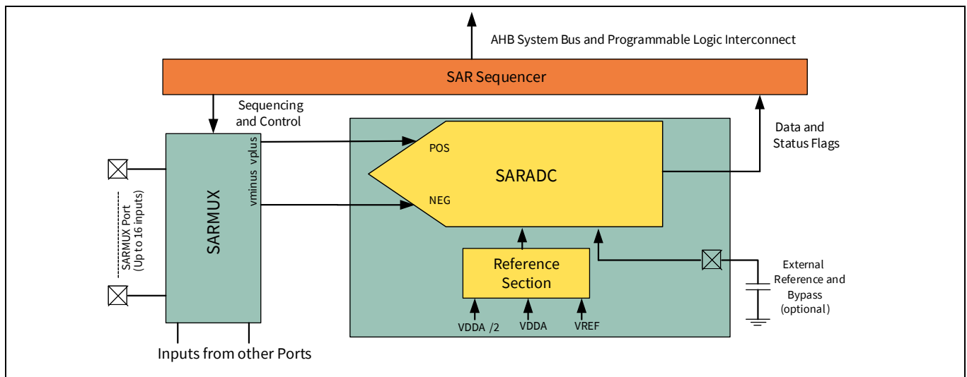
Figure 3 SAR ADC
