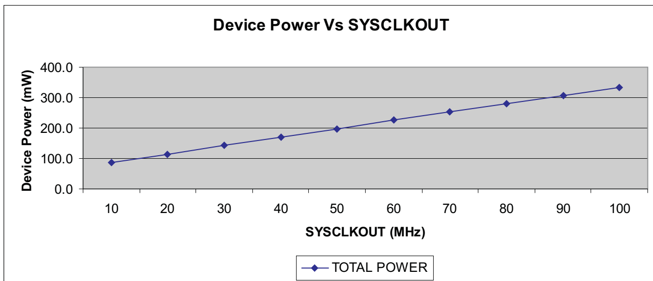
Figure 5-4. Typical Operational Power Versus Frequency (C280x)
