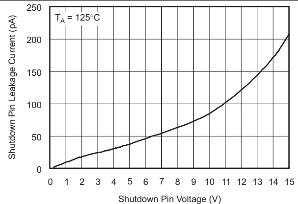
Figure 31. Shutdown Pin Leakage Current vs Shutdown Pin Voltage
