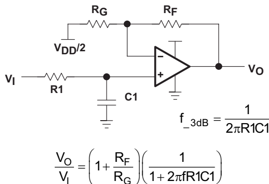
Figure 36. Single-Pole Low-Pass Filter
