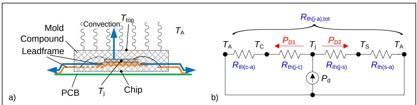
Figure 1 a) Cross section through an IC and package b) Thermal equivalent circuit
