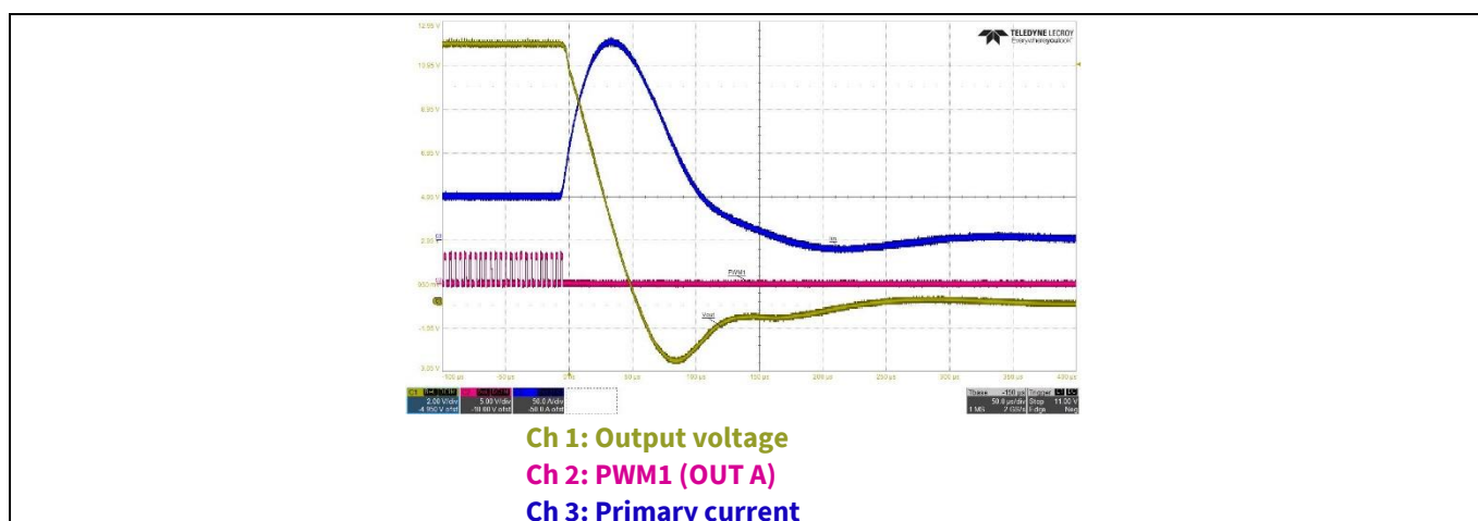
Figure 40 Short-circuit protection
