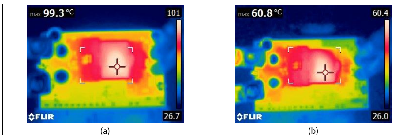
Figure 5 Thermal performance with V_{IN} = 48\text{ V} and I_{OUT} = 25\text{ A} - a) natural airflow, b) fan cooling
