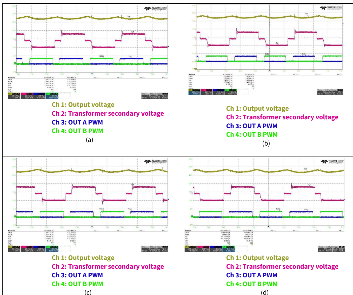
Figure 52 Flux balancing steady-state result - a) ramp0_dutyc_lock = unchecked (flux balancing disabled), b) ramp0_dutyc_lock = checked and I_{OUT} = 10 A (flux balancing is disabled due to DCM), c) ramp0_dutyc_lock = checked and fbal_time_only = enable (flux balancing is disabled due to DCM), d) ramp0_dutyc_lock = checked and fbal_time_only = disable (flux balancing enabled with volt \times seconds technique)
