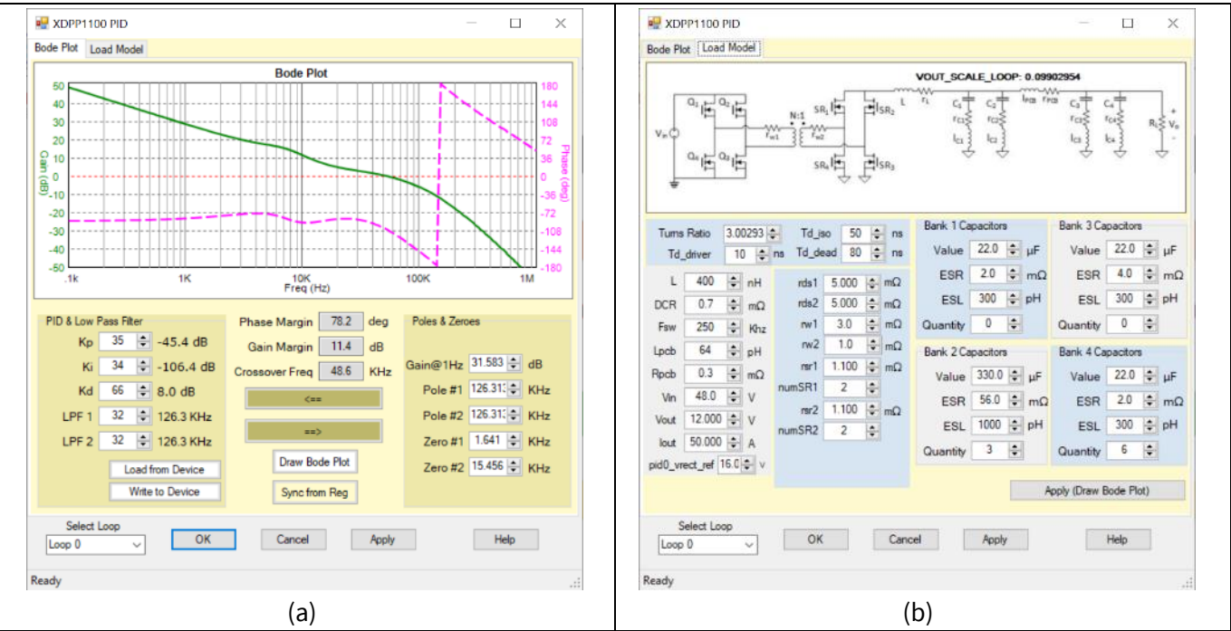
Figure 28 PID – bode plot - a) bode plot, b) load model
