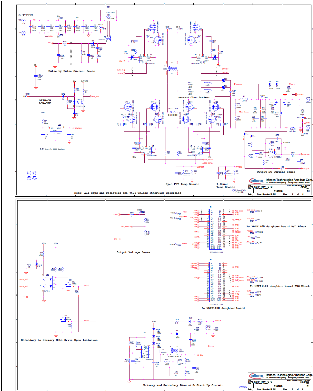
Figure 63 Power board schematic
