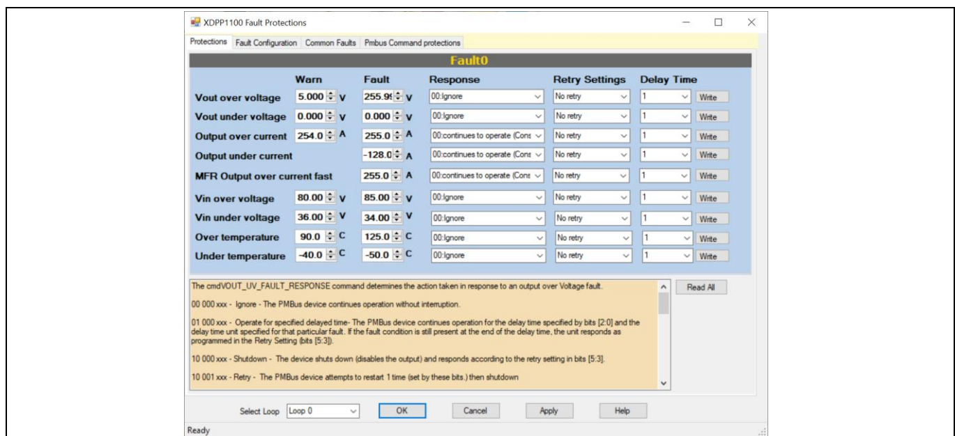
Figure 32 XDPP1100 fault protections window with Protections, Fault Configuration, Common Faults, and Pmbus Command protections tabs
