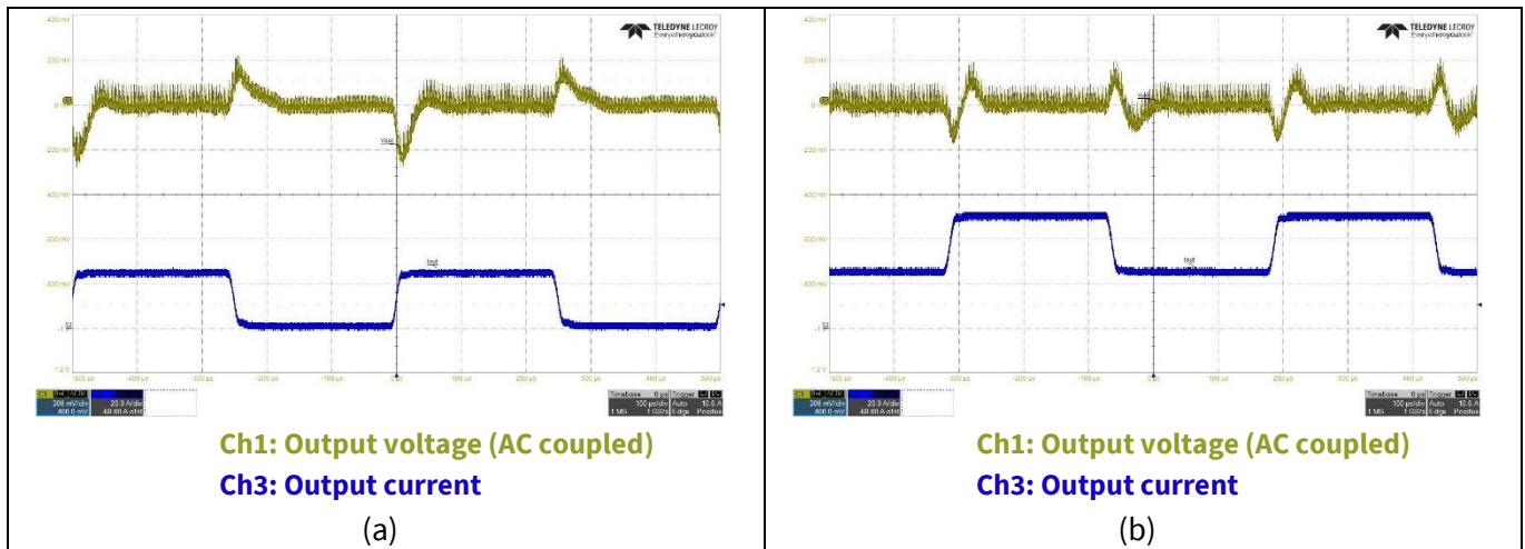
Figure 30 Load-transient response at V_{IN} = 48\text{ V} - a) load step: 5 percent ↔ 50 percent, b) load step: 50 percent ↔ 100 percent
