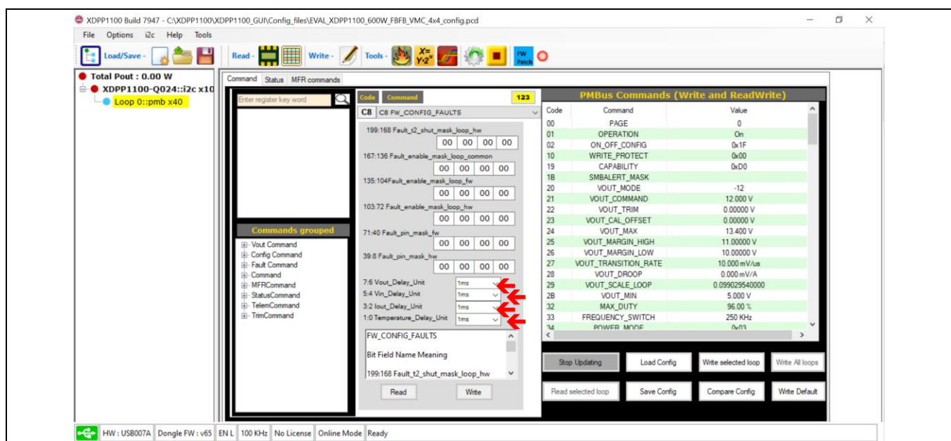
Figure 34 Setting Fault Delay Unit(s) in FW CONFIG FAULTS (Code C8) PMBus command
