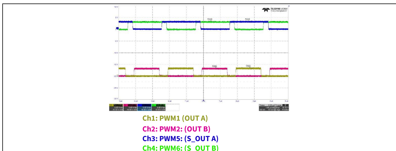
Figure 20 Evaluation kit PWM waveforms for 12 V DC output voltage and 10 A load current
