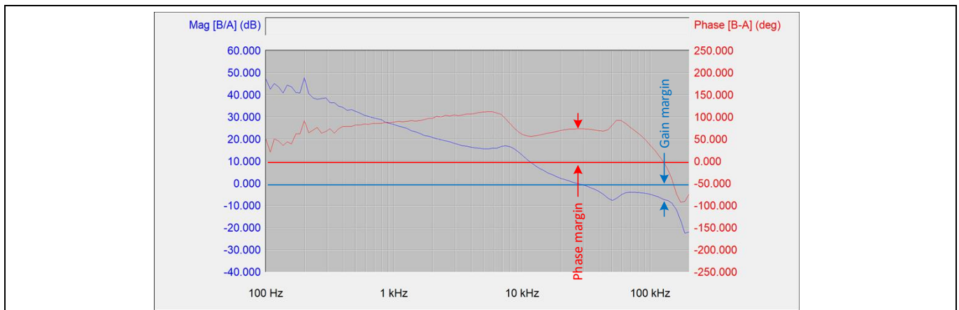
Figure 29 Experimental bode plot (phase margin = 75°, gain margin = 9 dB, crossover frequency = 28 kHz)
