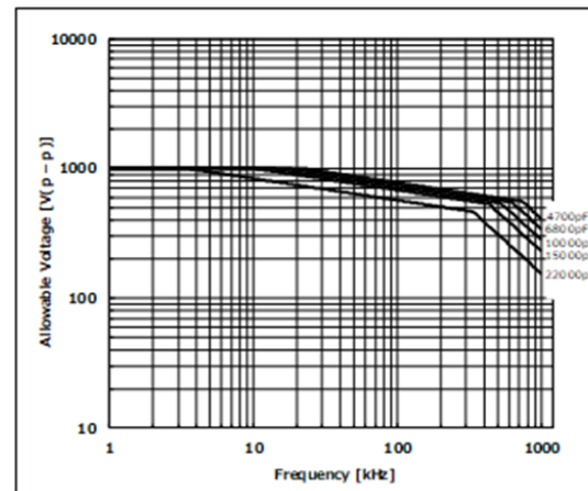
Chip(L×W): 3.2×2.5mm C0G(5C) Char. Rated Voltage:DC1KV
