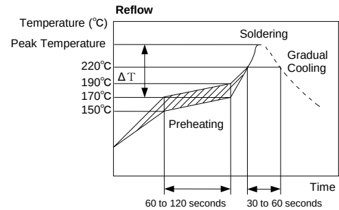
[Allowable Reflow Soldering Temperature and Time]
