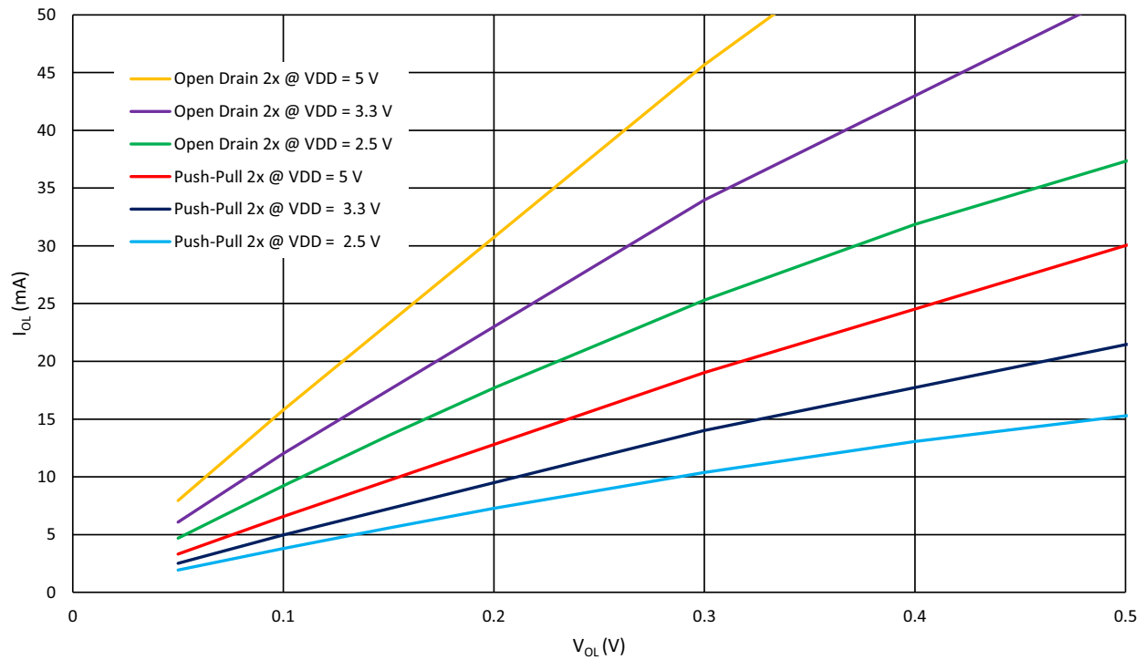
Figure 12: Typical Low Level Output Current vs. Low Level Output Voltage, 2x Drive at T = 25^\circ\text{C}
