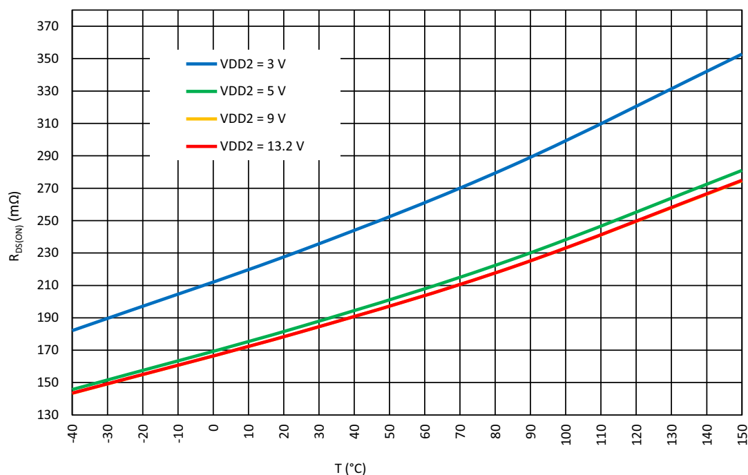
Figure 24: Full Bridge Typical Drain-Source Low Side On-Resistance vs. Temperature at I_{LOAD} = 0.5\text{ A} , V_{DD} = 5.5\text{ V}
