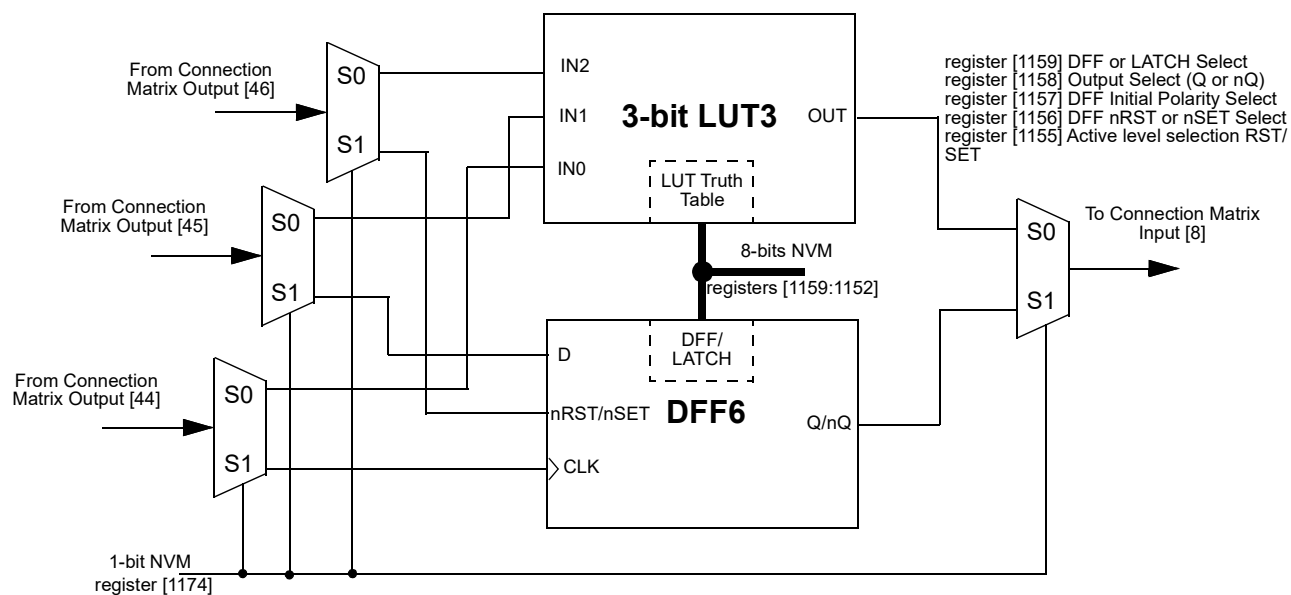
Figure 55: 3-bit LUT3 or DFF6
