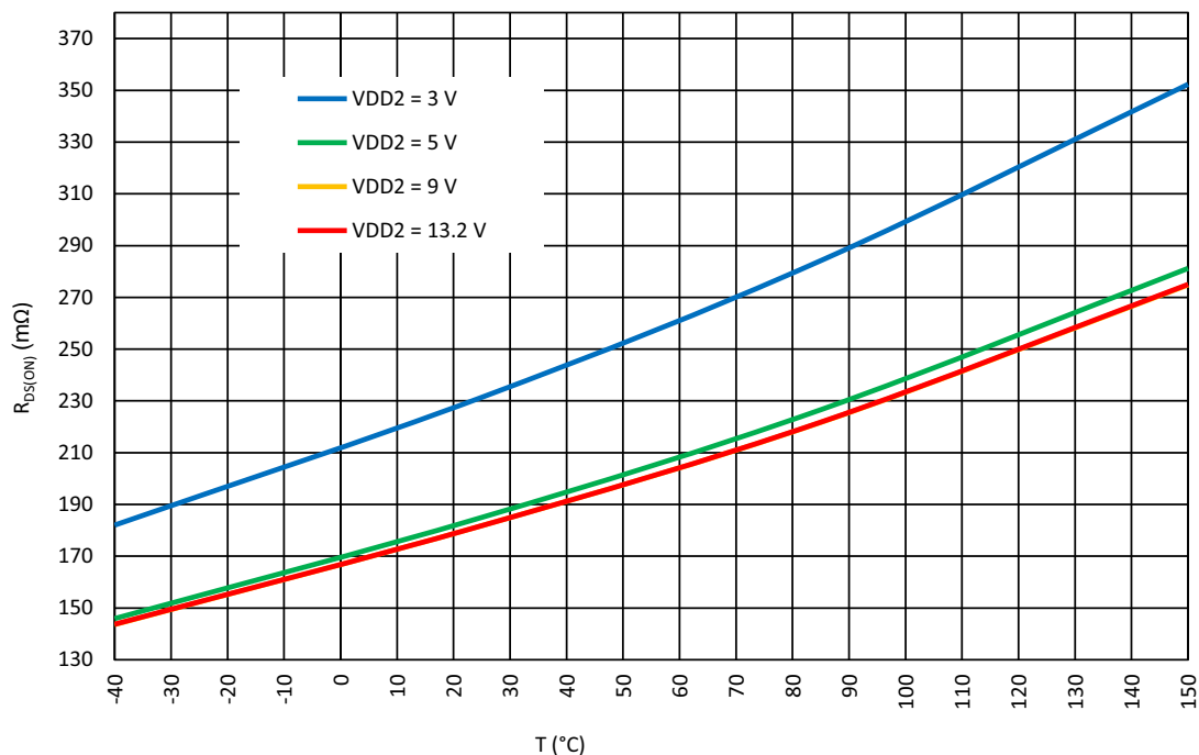
Figure 23: Full Bridge Typical Drain-Source Low Side On-Resistance vs. Temperature at I_{LOAD} = 0.5\text{ A} , V_{DD} = 2.3\text{ V}
