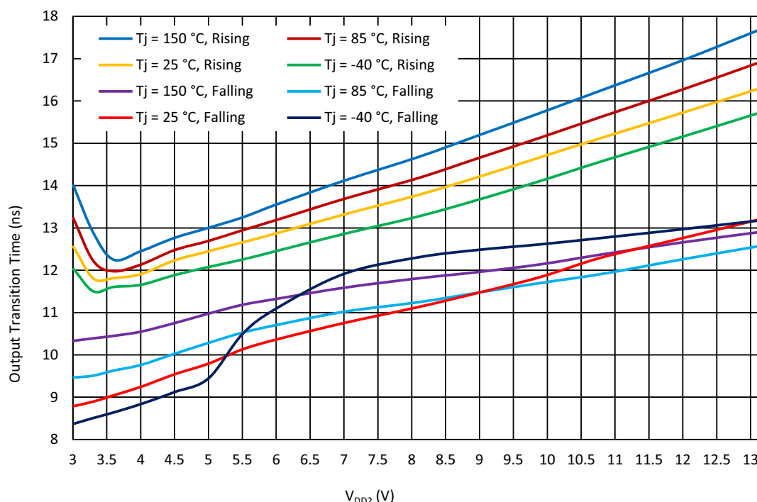
Figure 32: Half Bridge Output Transition Time vs. V_{DD2} at V_{DD} = 2.3 V to 5.5 V, f = 50 kHz for Pre-Driver Mode
