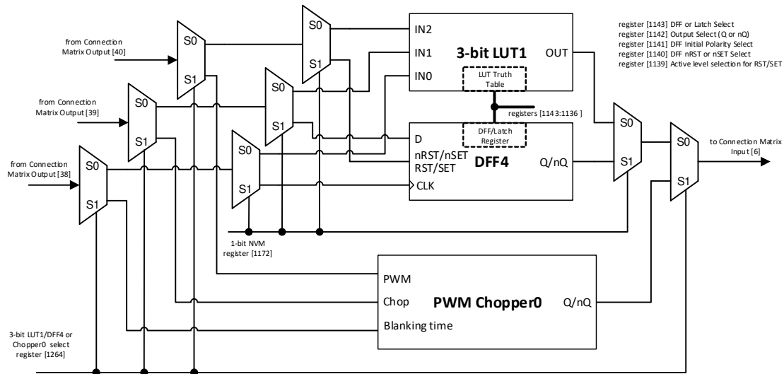
Figure 60: 3-bit LUT1 or DFF4
