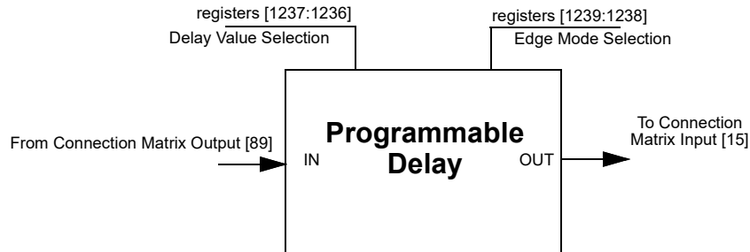
Figure 118: Programmable Delay
