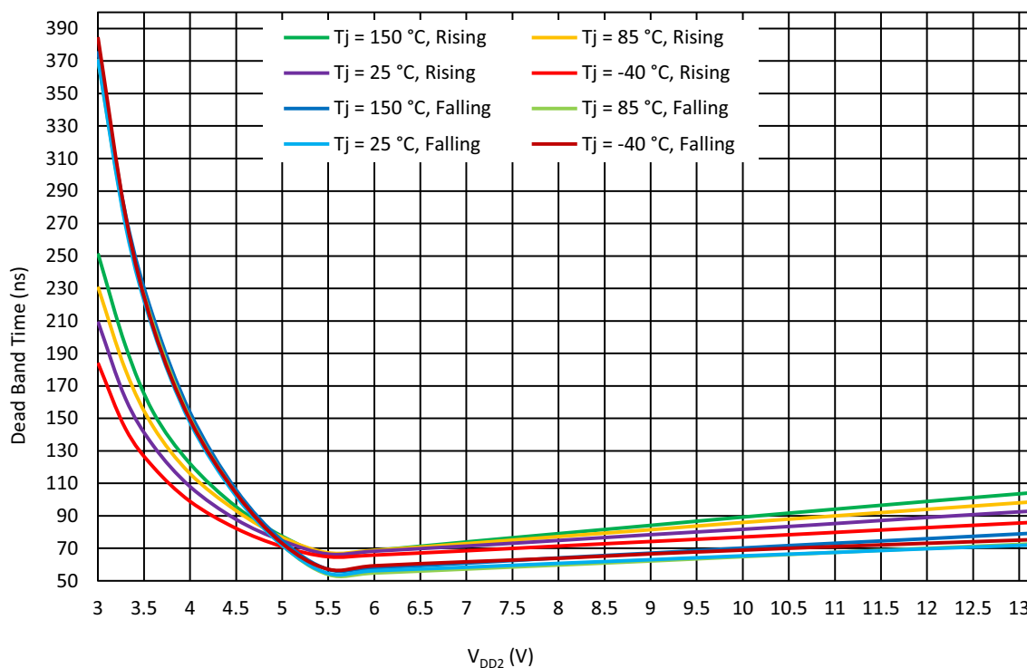
Figure 31: Half Bridge Dead Band Time vs. V_{DD2} at V_{DD} = 2.3 V to 5.5 V, f = 50 kHz for Regular Mode
