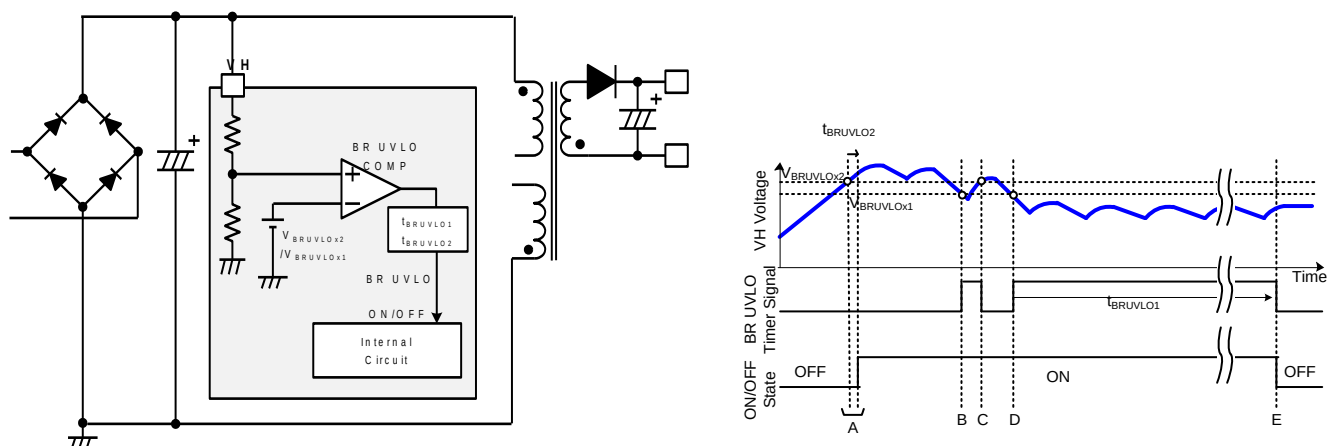
Figure 4. BR UVLO Block Diagram and Timing Chart
