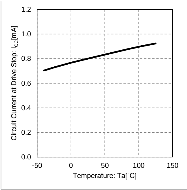
Figure 21. Circuit Current at Drive Stop vs Temperature
