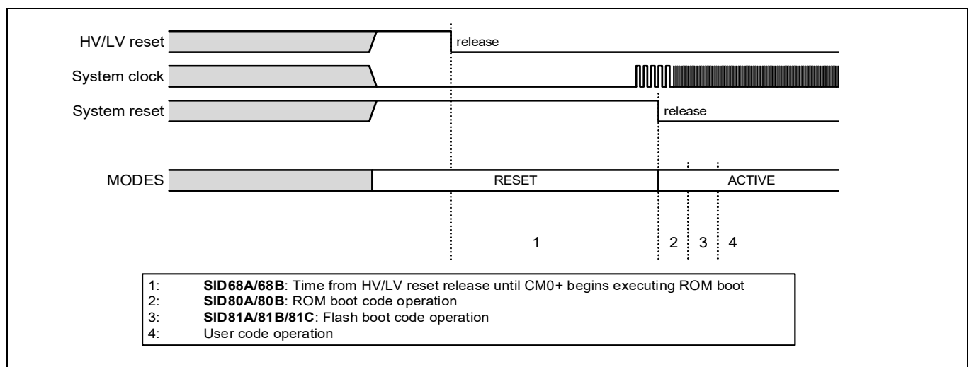
Figure 26-3 Reset sequence
