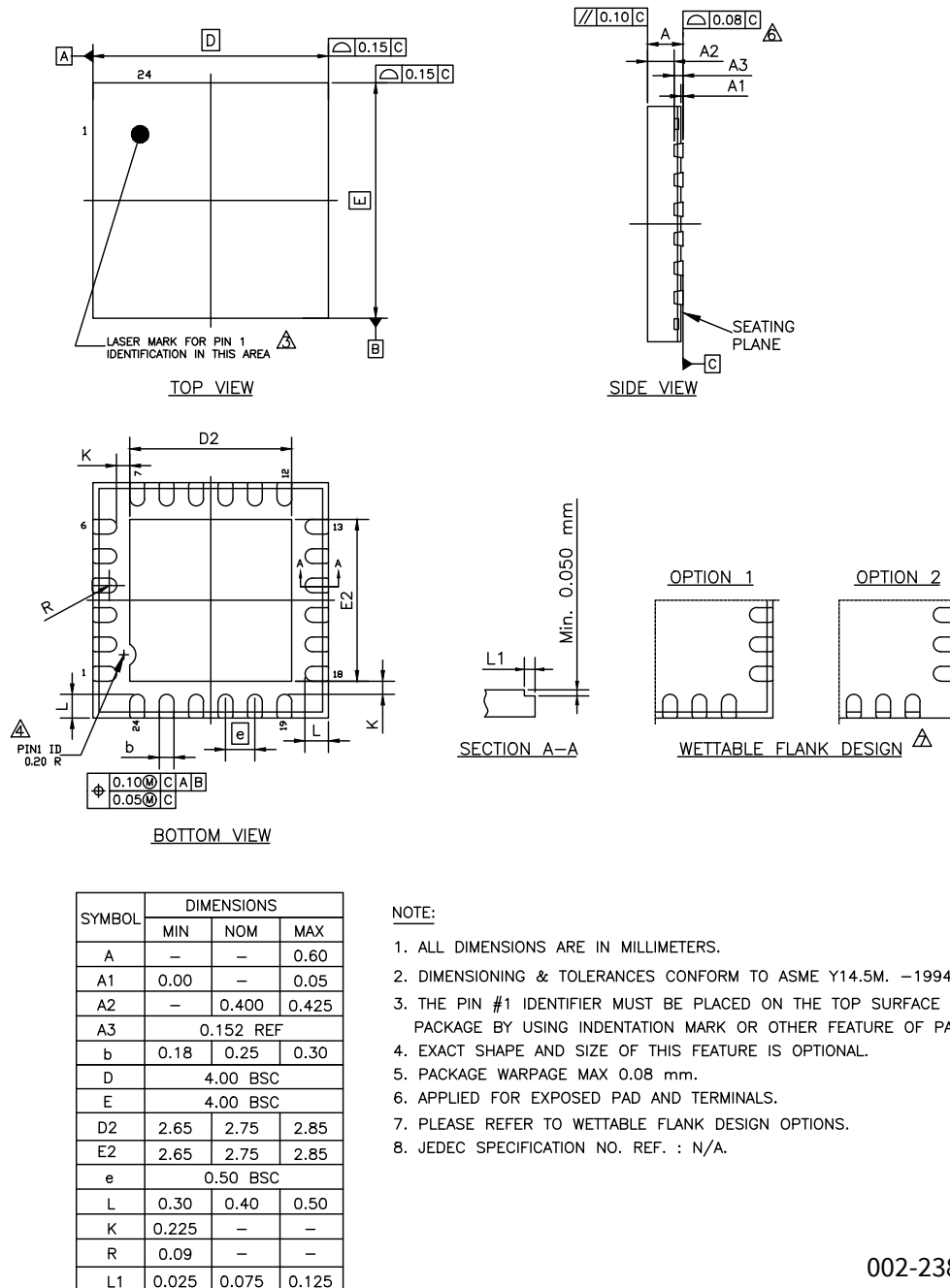
Figure 7 24-pin QFN package outline (PG-VQFN-24)
