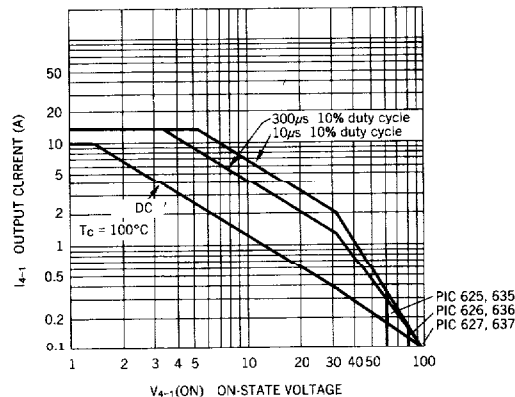
Maximum Safe Operating Area PIC 625, 626, 627-635, 636, 637
