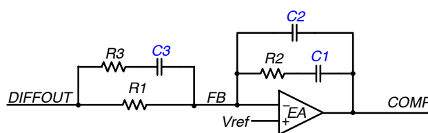
Figure 10. Error Amplifier
