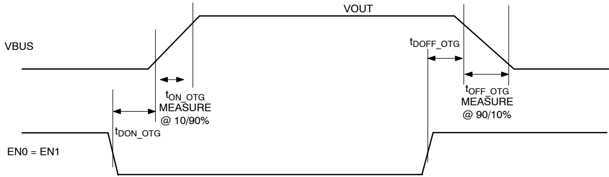
Figure 9. OTG Mode Operation (VOUT = 5 V, VPWR_SIG > UVLO)
