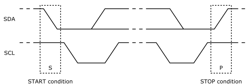
Figure 6. Start and Stop Condition on the I 2 C Bus
