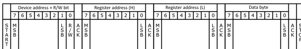
Figure 9. Interface protocol
