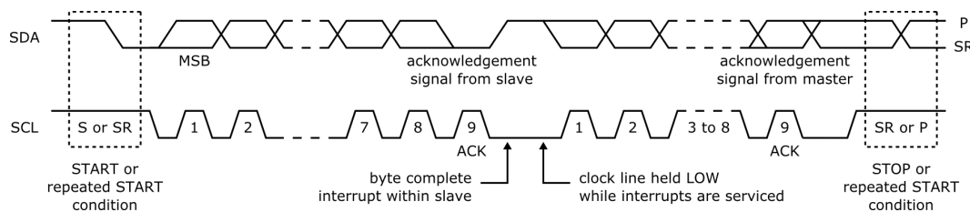
Figure 7. Byte transfer
