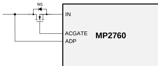
Figure 4: ACGATE Driver
