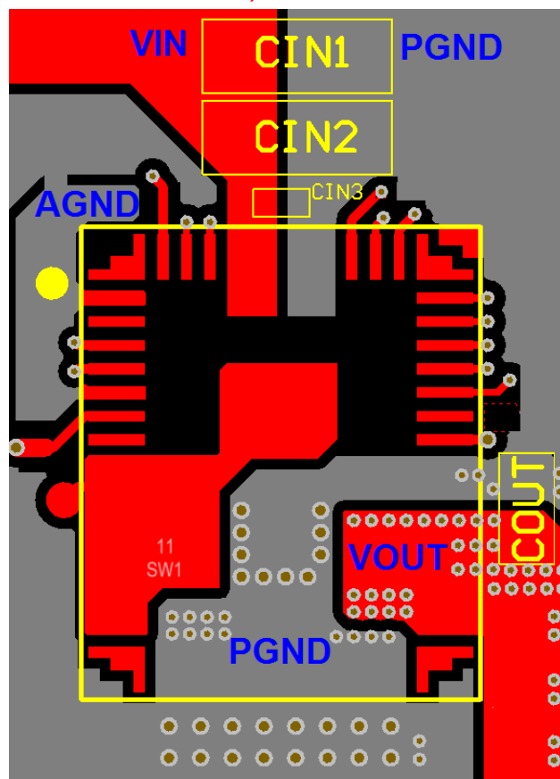
Figure 4. Example Layout - Top Layer
