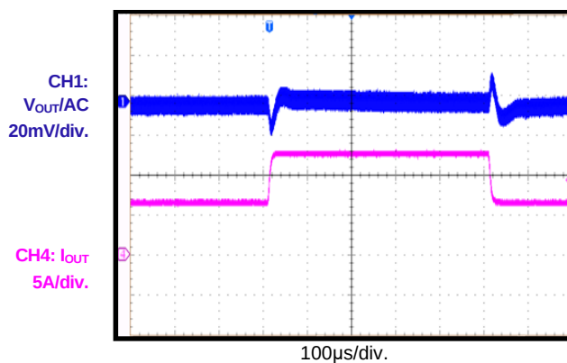
Load Transient
