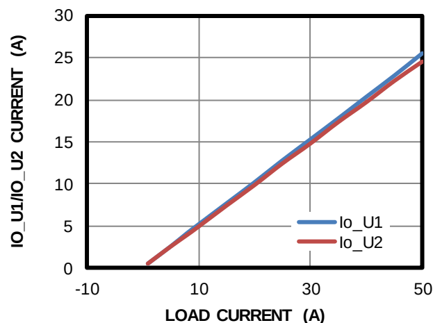
Current Sharing
