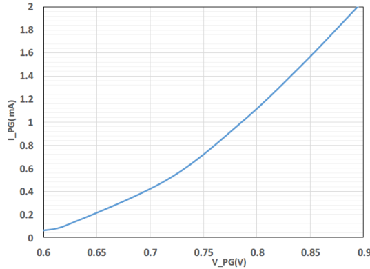
Figure 3: Power-Good Current vs. Power-Good Voltage
