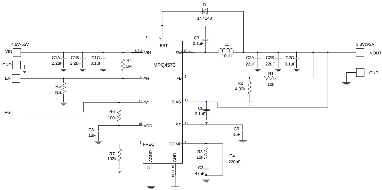
Figure 4 – 3.3V Output Typical Application Circuit
