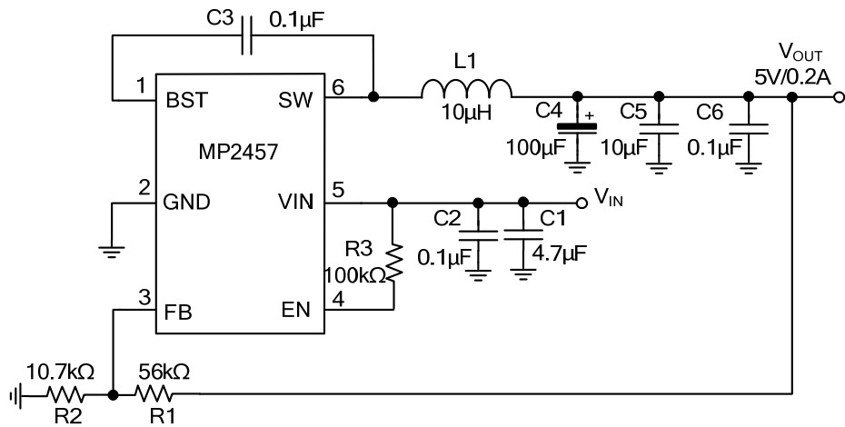
Figure 5: 5V Output
