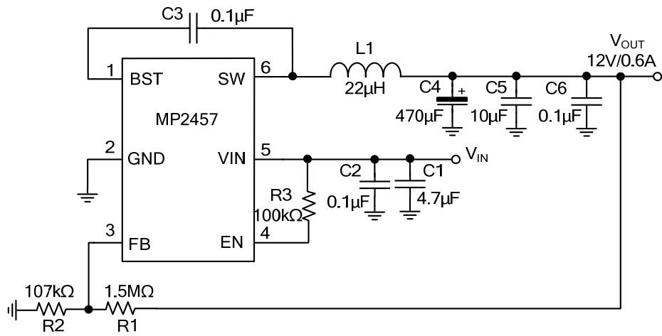
Figure 4: 12V Output
