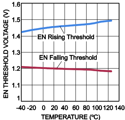
V_{EN} Threshold vs. Temperature
