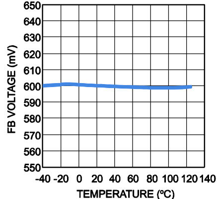
V_{FB} Voltage vs. Temperature
