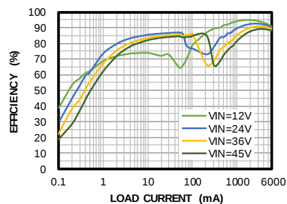
Efficiency vs. Load Current V_{OUT}=3.3V , F_{SW}=470kHz , L=3.3\mu H , AAM
