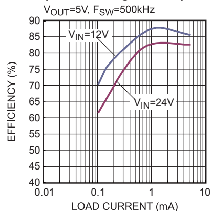
Efficiency vs. Load Current (Extreme Light Load)
