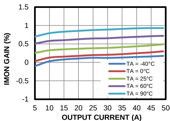
IMON Gain vs. Output Current
