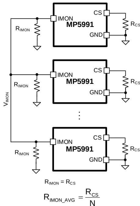
Figure 16: IMON and CS Connections in Multi-Fuse Parallel Application
