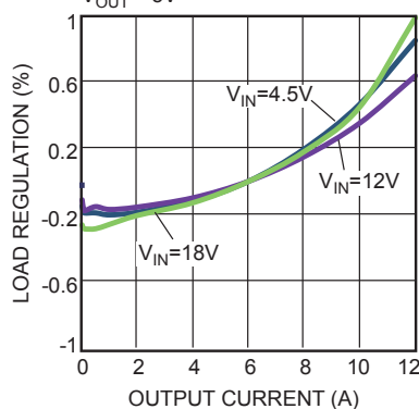
Load Regulation vs. Output Current V_{OUT} = 5V
