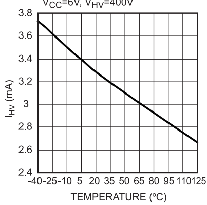
Supply Current from HV vs. Temperature V_{CC}=6V, V_{HV}=400V
