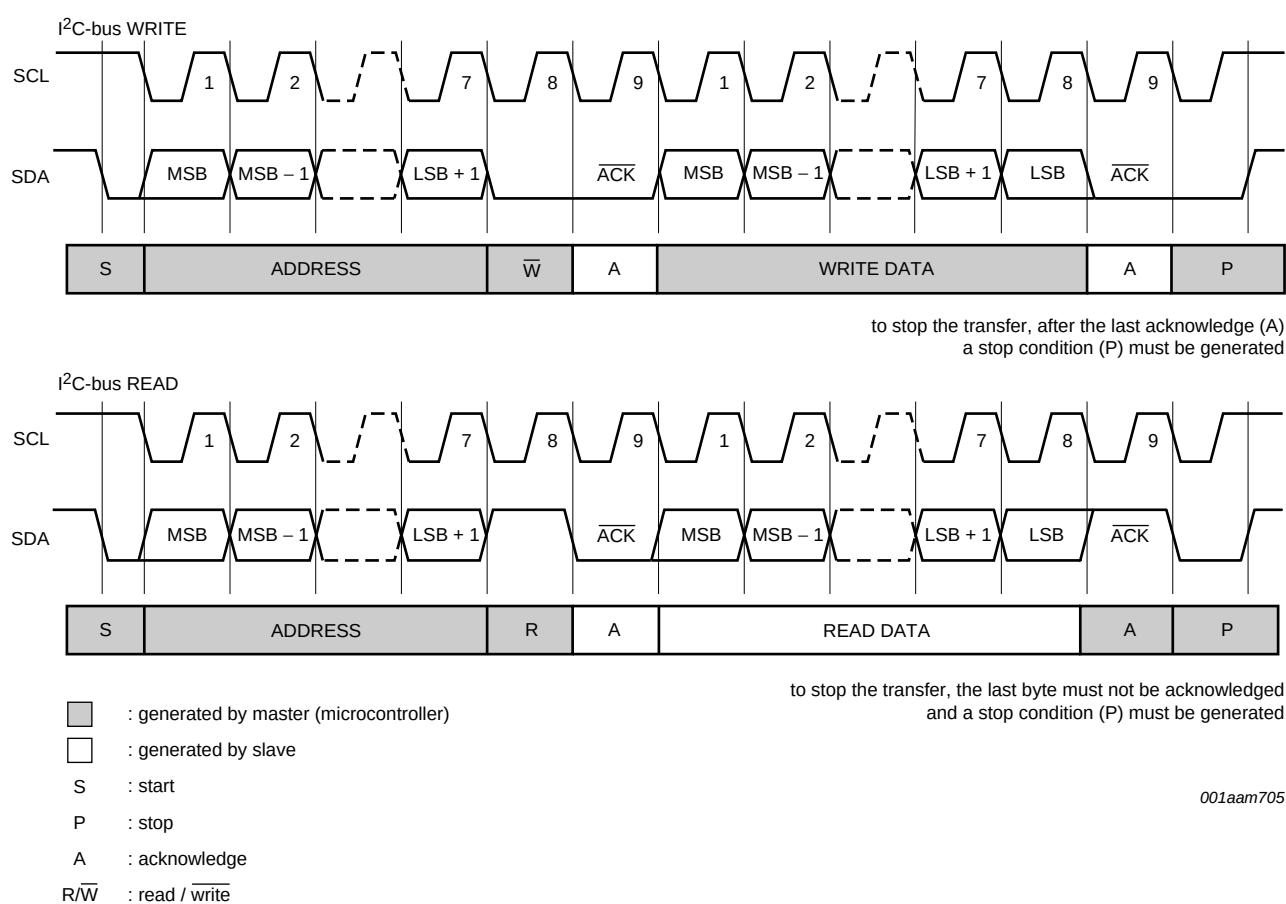
Fig 18. I 2 C-bus read and write modes
