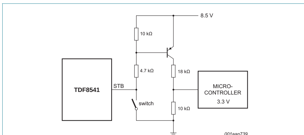
Fig 31. Circuit for testing clip detection on pin STB
