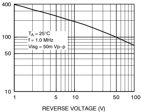
Figure 5. Junction Capacitance
