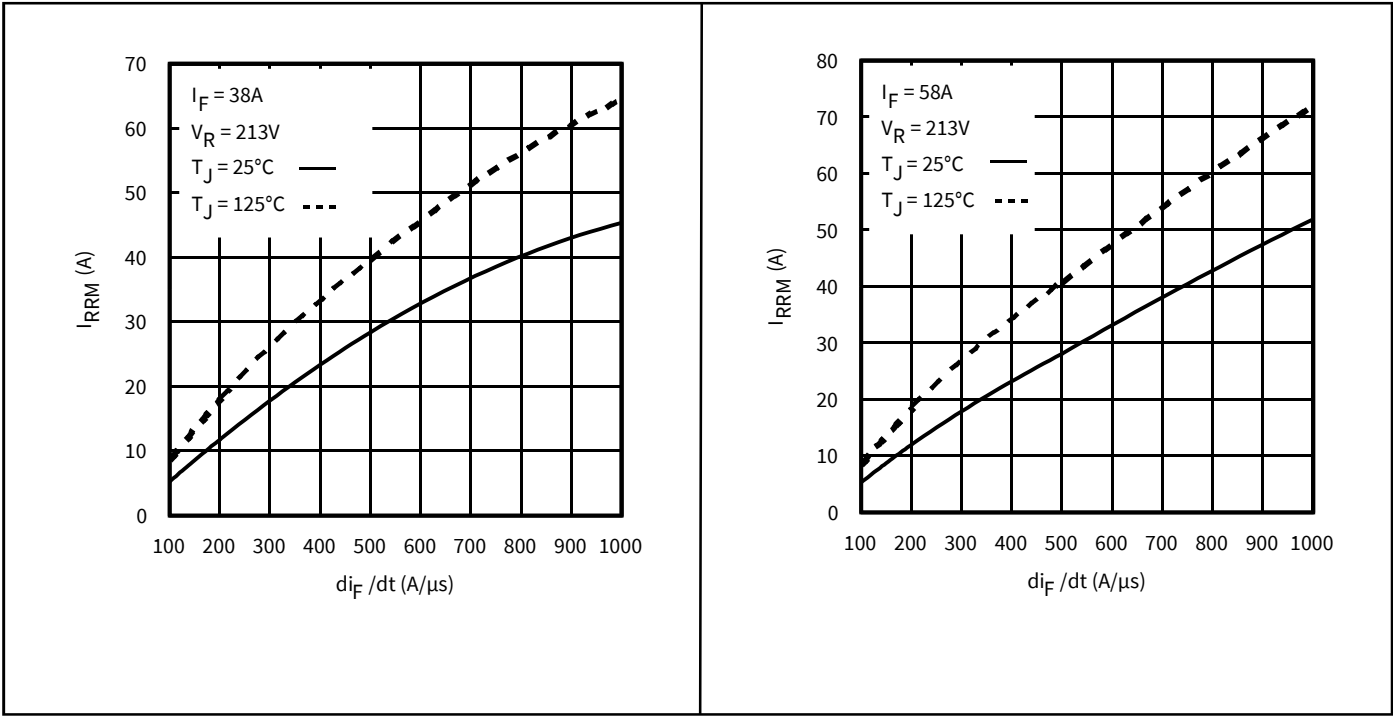
Figure 18 Typical Recovery Current vs. di_F/dt
