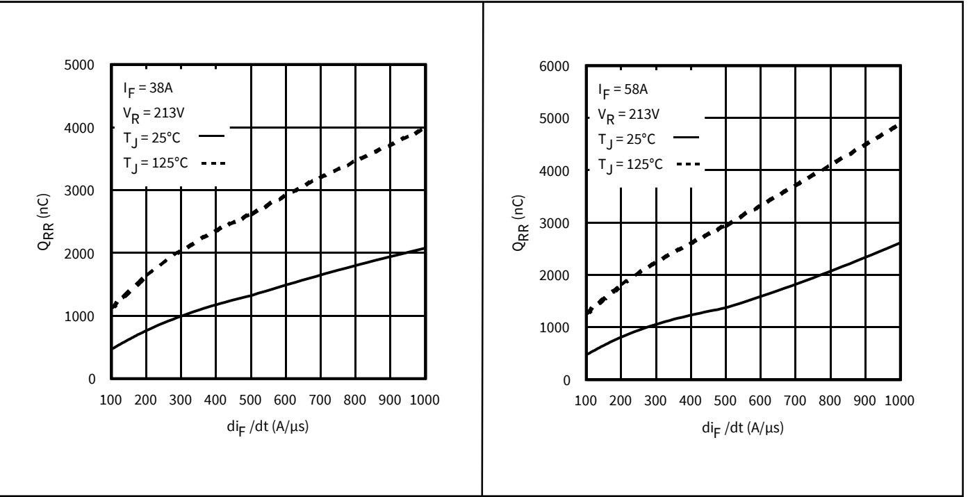
Figure 20 Typical Stored Charge vs. di_F/dt
