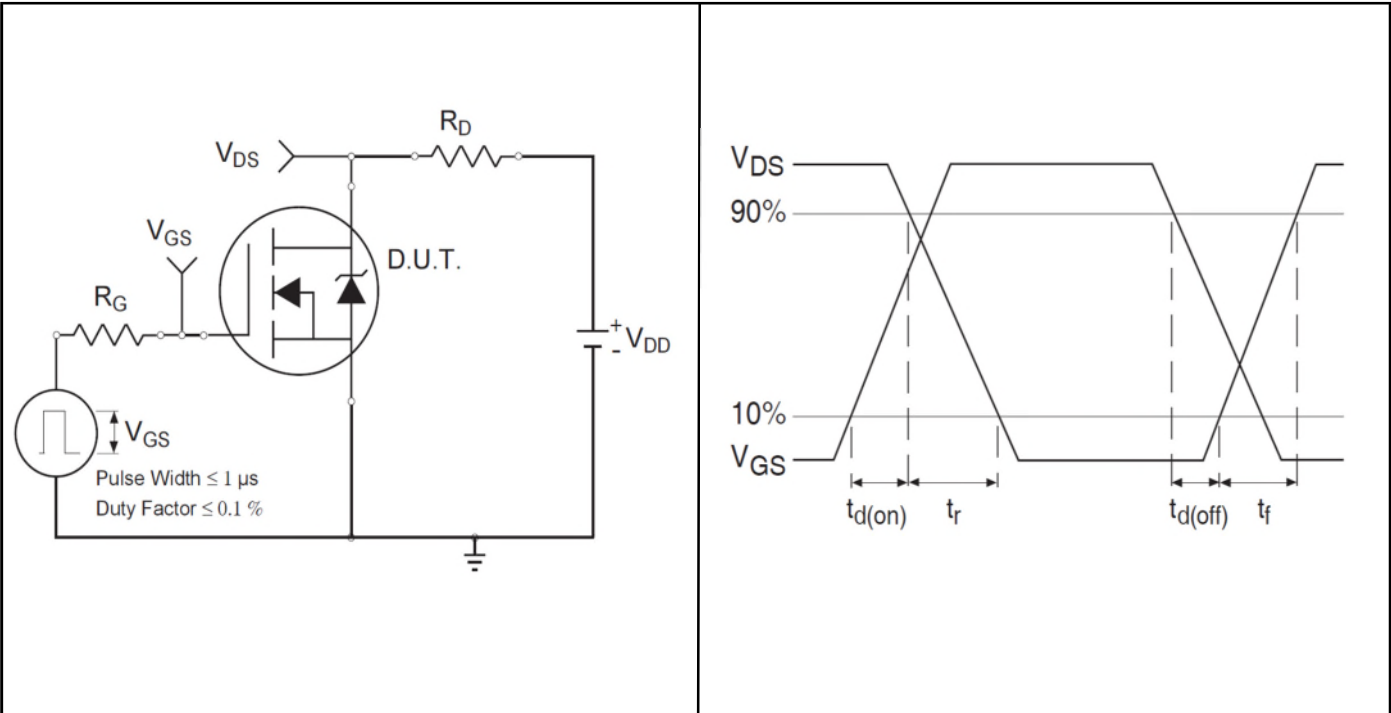
Figure 24a Switching Time Test Circuit
