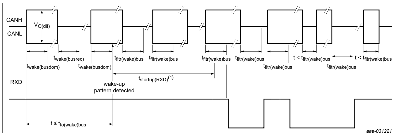
Figure 6. Wake-up timing
