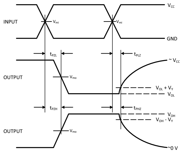
Figure 4. Switching Waveforms
