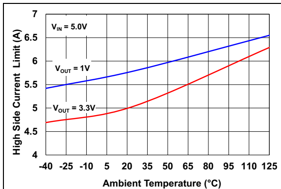
FIGURE 2-3: High-side Current Limit vs. Temperature.
