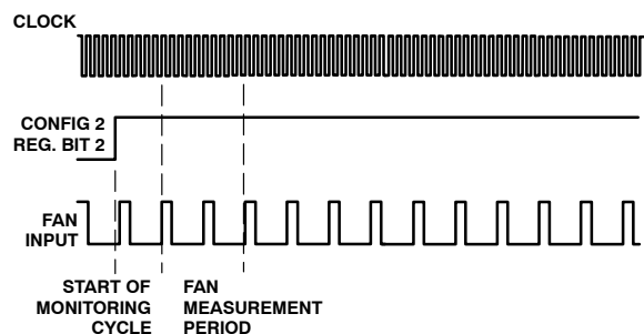
Figure 37. Fan Speed Measurement
