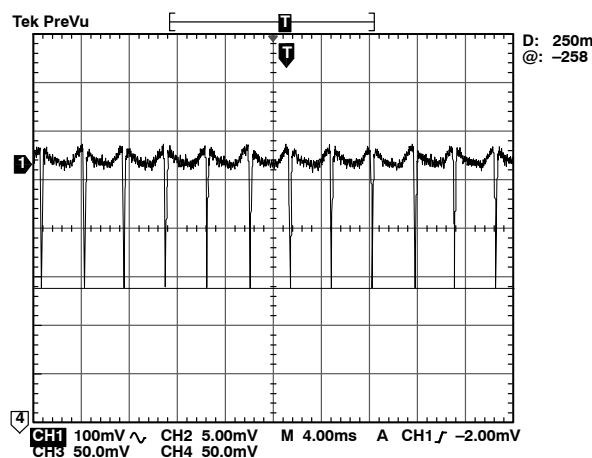
Figure 36. Fan Speed Sensing Waveform at TACH/AIN Pin
