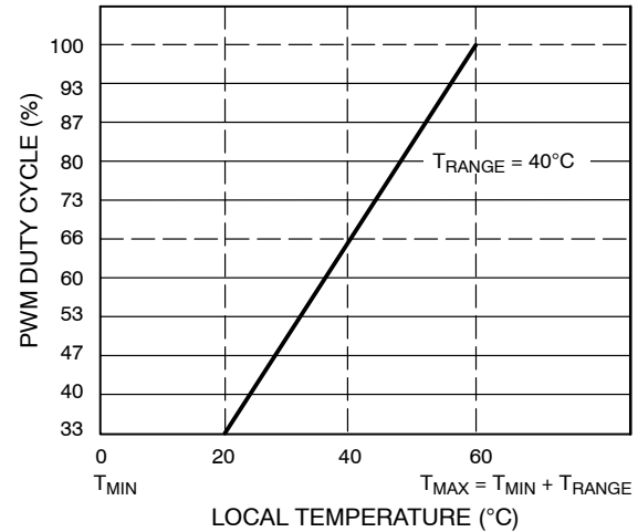
Figure 24. Max Speed Calculated by Local Temperature Control Loop Drives Fan
