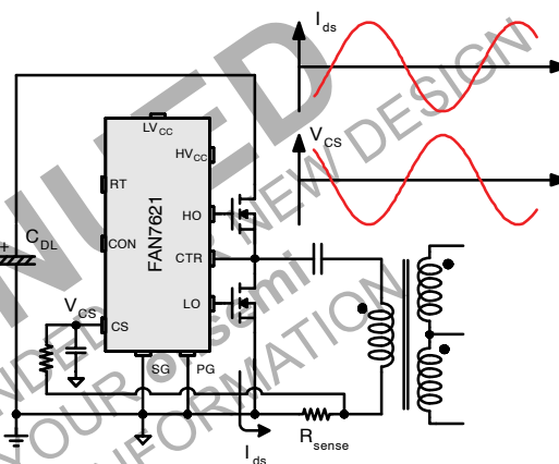
Figure 26. Full-Wave Sensing
