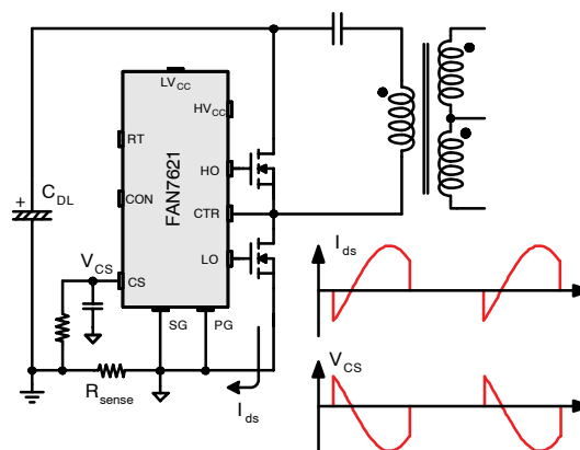
Figure 25. Half-Wave Sensing
