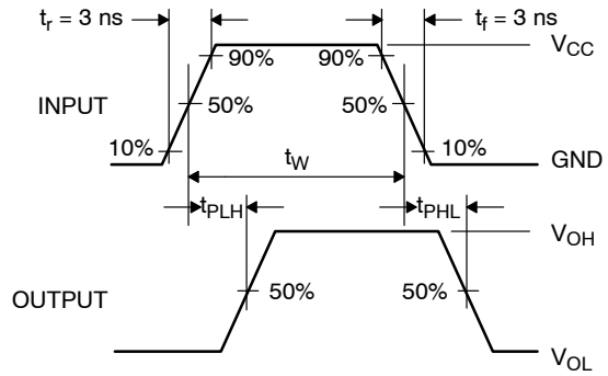
Figure 7. AC Waveforms
