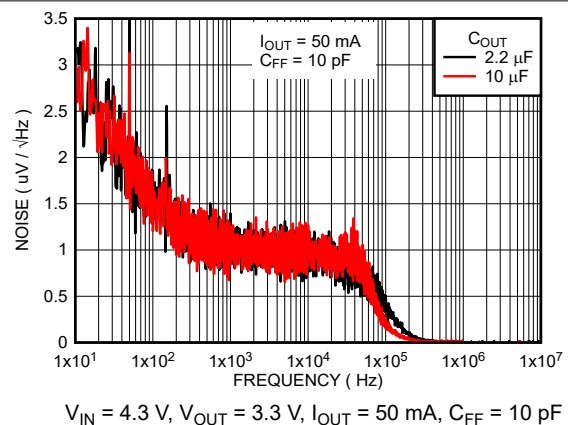
Figure 6-36. Output Noise Density vs C_{OUT} for New Chip
