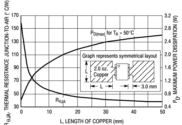
Figure 8. SOIC-8 Thermal Resistance and Maximum Power Dissipation versus P.C.B. Copper Length
