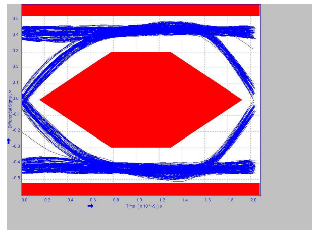
Figure 9-15. 1 Meter Post-Channel With TUSB217A BOOST=0 RX_SEN=MED
