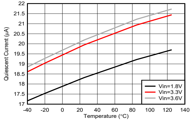
Figure 7-7. Quiescent Current into VIN vs Temperature
