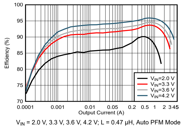
Figure 7-2. Efficiency vs Output Current V_{OUT} = 5\text{ V}
