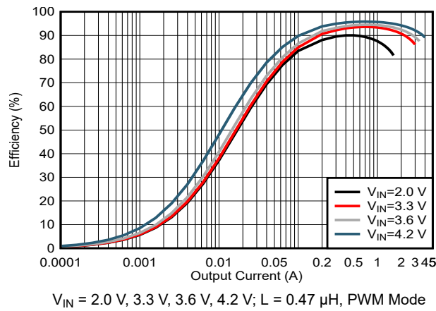
Figure 7-1. Efficiency vs Output Current V_{OUT} = 5\text{ V}
