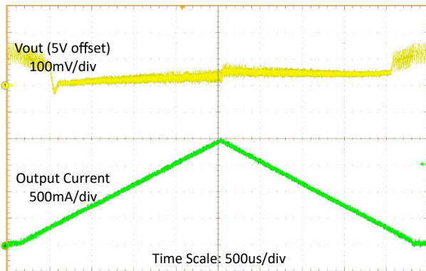
Figure 9-8. Load Sweep
