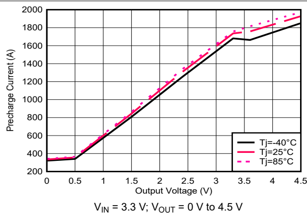
Figure 7-5. Pre-charge Current vs Output Voltage
