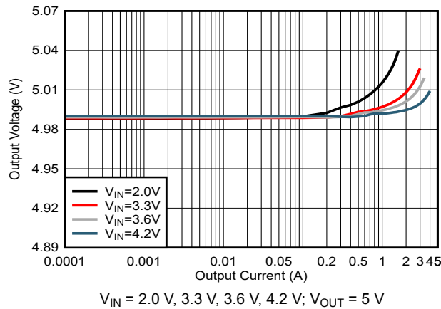
Figure 7-3. Load Regulation in Auto PWM
