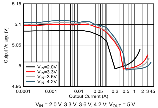
Figure 7-4. Load Regulation in Forced PFM
