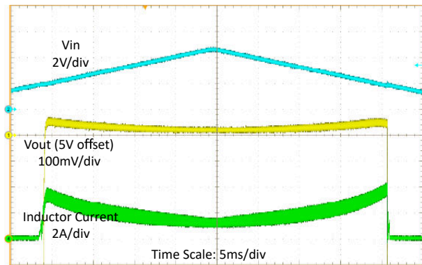
Figure 9-9. Line Sweep
